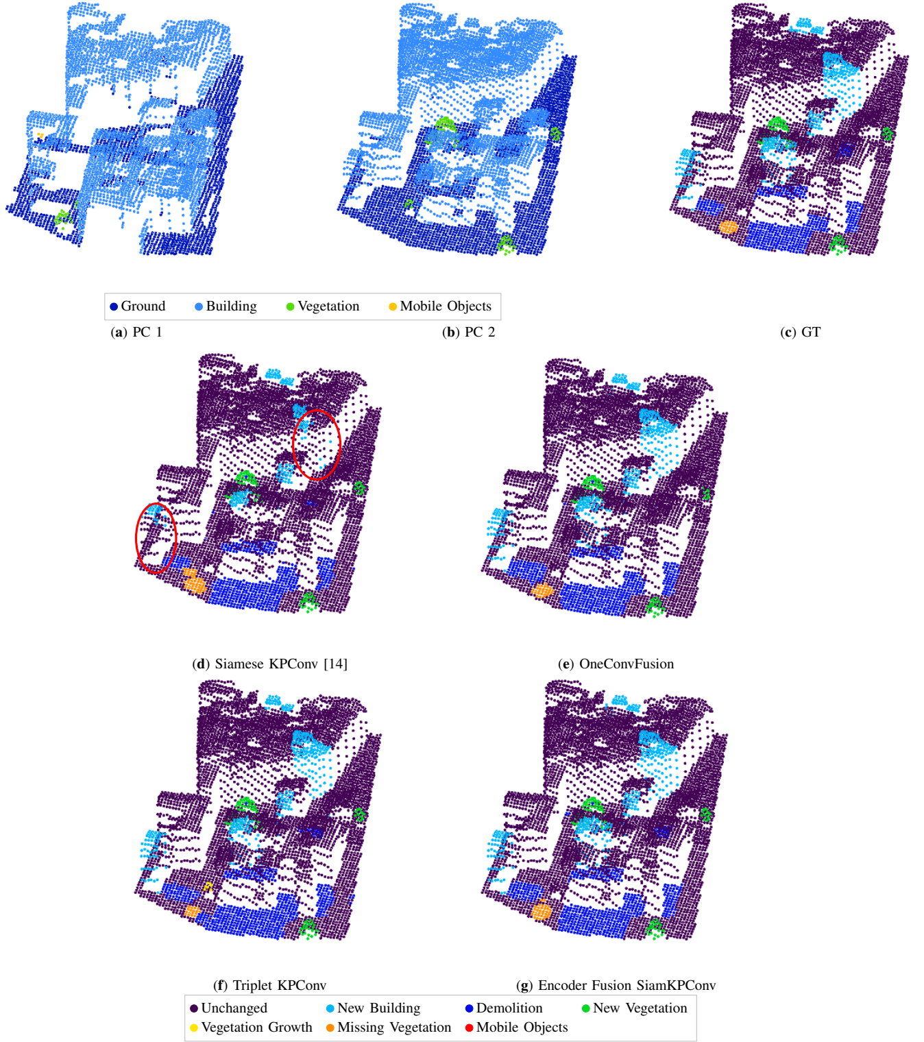
Fig. 7. Visual change detection results on Urb3DCD-V2 low density LiDAR sub-dataset in an area containing occlusions: (a-b) the two input point clouds; (c) ground truth (GT); simulated changes; (d) Siamese KPConv results; (e) OneConvFusion results; (f) Triplet KPConv results; (g) Encoder Fusion SiamKPConv results. Regions of interest specifically discussed in the text are highlighted with ellipses.
