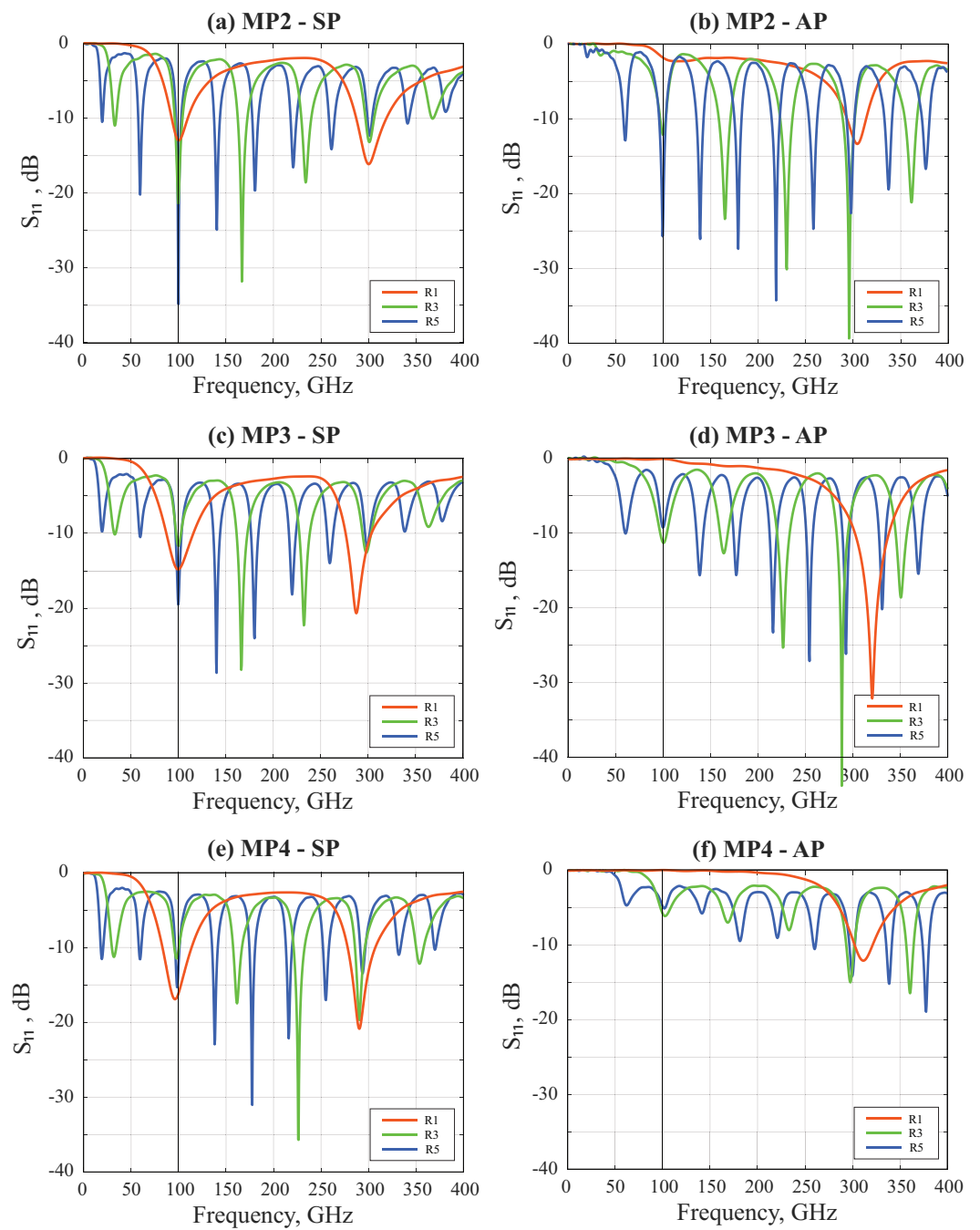
Figure 4. S_{11} simulation of the multipolar antennas MP2–MP4, for resonance orders R1, R3, and R5. (Left) Super-dipole multipin polarity excitation (SP). (Right) Alternate-polarity excitation (AP).
