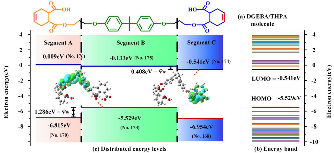
Fig. 2. The energy band structure and distributed energy levels of DGEBA/THPA molecule
