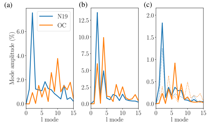
FIG. 2: N190204-003 (N19, blue) and Optimized Config (OC, orange) spherical harmonics “ l modes” for: (a) illuminations without an ablation plasma, related to Figure 1b; (b) ablation pressures from Equation 1 generated with plasma and CBET, related to Figure 1c; and (c) target areal densities at \approx 9\text{ns} . Mode amplitudes are given as a percentage of the mean. The dotted lines in (c) are a combination of (a) and (b) in quadrature.
