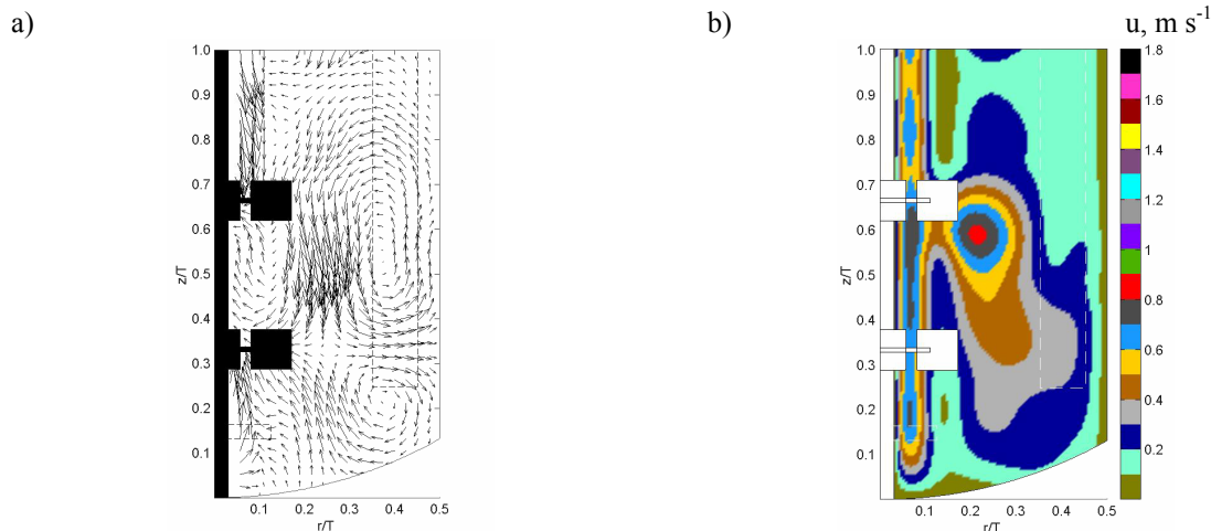
Figure 2. Measurements in the plane r - z , midway between the baffles in the single liquid phase agitation system with dual – impellers of the same dimensions: a) 2–D map of mean velocity vectors, b) Contours of three component fluctuating velocities.
