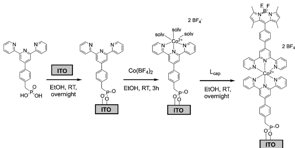
Scheme 1. Synthetic method followed for the anchoring of the functional complex [(L_a)Co^{II}(L_c)](BF_4)_2 on ITO ( L_c = BODIPY-Ph-tpy and L_a = O_3P-CH_2 -Ph-tpy).
