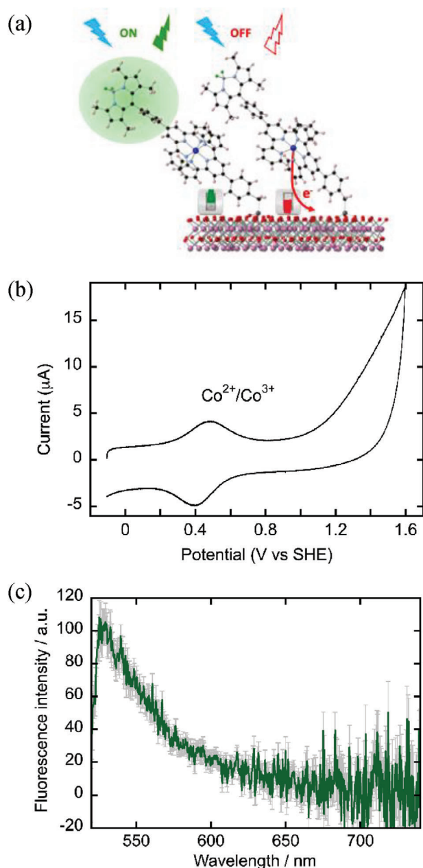
Figure 1. a) Illustration of the concept based on functional monolayers of [(\text{L}_a)\text{Co}^{\text{II}}(\text{L}_c)](\text{BF}_4)_2 covalently immobilized on the ITO electrode; b) Cyclic voltammogram of the monolayer ITO- [(\text{L}_a)\text{Co}^{\text{II}}(\text{tpy-Ph-BODIPY})] (in \text{CH}_3\text{CN}/\text{Bu}_4\text{N}^+\text{PF}_6^- (0.1 M), 25 °C); c) Corrected fluorescence emission spectra (—, green) and its corresponding amplitude standard deviation (—, grey) at the monolayer-electrolyte interface averaged within 2 sec after the start of the laser irradiation at 474 nm.
