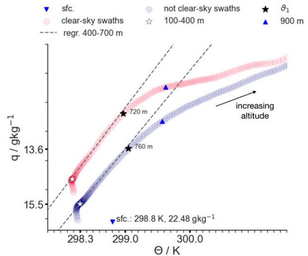
FIG. 11. As in Fig. 10, but for q and \theta soundings aggregated for large clear-sky areas (red) and areas influenced by cloudiness (blue, following the conditional sampling in Fig. 6). Also shown are the campaign-mean surface value (blue downward triangles), value averaged from 100 to 400 m (white stars), \vartheta_1 value annotated with its height (black stars), and value at 900 m (blue upward triangles). Data-derived mixing lines are linear regressions to the observed profile from 400 to 700 m (gray dotted lines).
