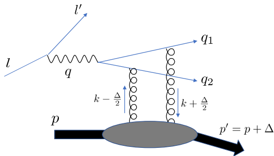
Fig. 1. Exclusive dijet production in ep collisions.
