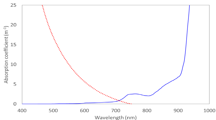
Figure 10. Absorption coefficient of CDOM from lake Nohipalu Mustjärv (red graph) and pure water absorption spectrum (blue line) [5].
