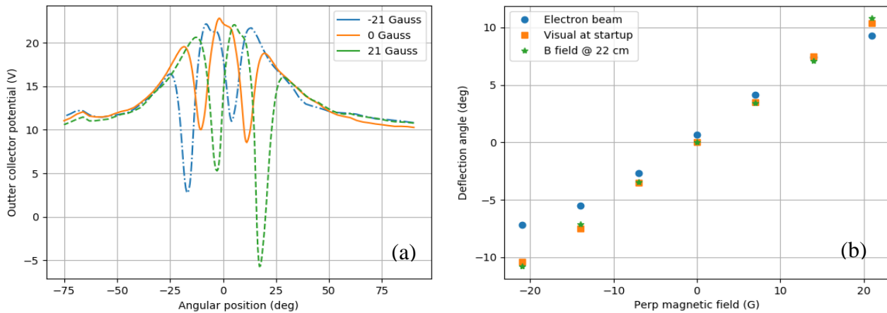
Figure 8: (a) Angular profile of the floating potential of the Faraday probe outer collector for three different fields: -21 , 0 , and +21 gauss. (b) Deflection angle of the electron beam against the applied B field.
