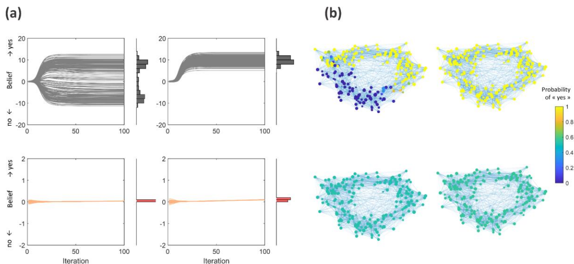
Figure 3. Response of an example 200-node small-world network ( K=20 , \beta=0.12 ) to uninformative external messages (random and unbiased). (a) Temporal evolution of the belief under the message passing algorithm (that is, while internal messages propagate in the network). By convention, the final beliefs are those obtained after 100 iterations. Two example trials are provided. Top row: BP leads to two possible outcomes depending on whether the whole population behaves similarly or separates into two groups with opposite, extreme beliefs. This is interpreted as polarization ( left ) or radicalization (unimodal in the right panel, bimodal in the left panel). Bottom row: In contrast, CBP leads to beliefs narrowly distributed around a weak consensus. This consensus varies from trial to trial but remains close to zero, reflecting higher uncertainty. (b) Final beliefs of the 200 nodes, visualized in the whole graph. The nodes (dots) are arranged topographically according to the path lengths (separation within the graph). The size of a dot represents the node's degree, and its color represents the marginal posterior probability estimate ( b(x_i = \text{“yes”}) ), abbreviated as the “Probability of yes”. Thin lines are connections. The two trials shown here are the same as in (a), with the top and bottom rows corresponding to BP/CBP. The relationship between the belief and the “probability of yes” is illustrated in Sup.Fig.1 .
