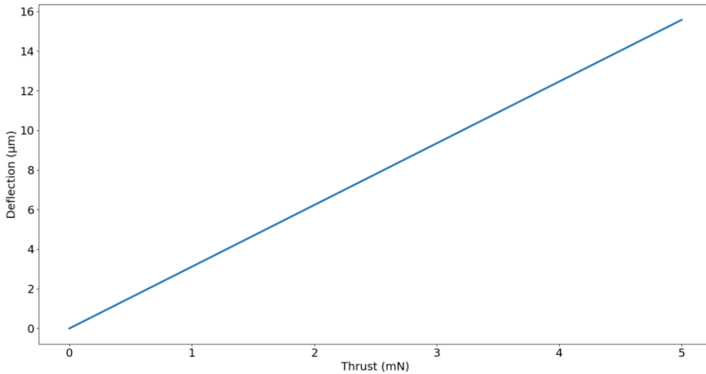
Figure 3: Platform deflection of the dual pendulum in response to a constant thrust. Geometrical parameters for the simulation: y_1 = 4 mm, y_2 = 4 mm, x_p = -10 mm, l = 15 cm, L = 19 cm and m_1 = m_2 = m_p = 4 kg. The Be-Cu strips dimensions: l_{strip} = 5 mm, w = 5 mm and e = 0.1 mm and Young's modulus E = 132 GPa .
