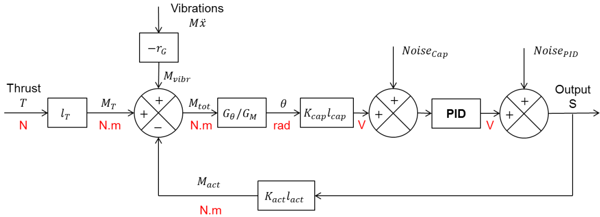
Figure 4: Block diagram of the nulled dual pendulum thrust stand.
