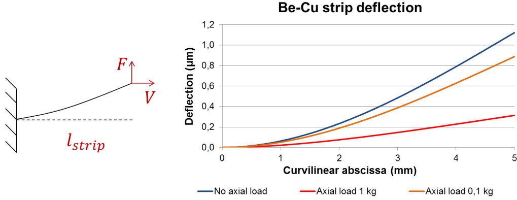
Figure 2: Be-Cu strip deflection under axial load V and transverse load F based on Eq. (1). The strips material is Beryllium-Copper, so E = 132 GPa, and the strips dimensions are l_{strip} = 5 mm, w = 5 mm and e = 0.1 mm. F = 1 mN.
