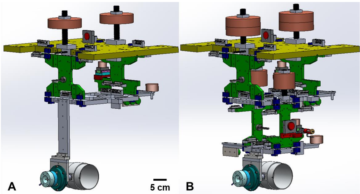
Figure 5: CAD model of the thrust stand concept. A) 1-axis dual pendulum TS. B) 2-axis TS. Yellow: Fixed platform. Blue: Be-Cu strips and fastening. Green: Arms with counterweights above the fixed pivots, one accelerometer per stage and one actuator. The calibration comb is also visible. Grey: Moving platform with capacitive sensor target and magnets for the damping and the actuation. The ECR thruster is at the bottom.
