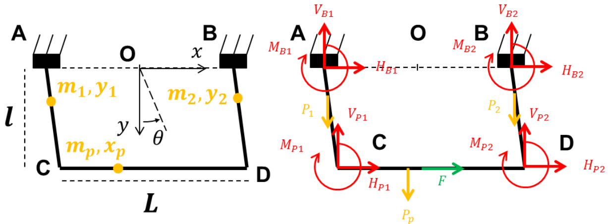
Figure 1: Mechanical system of a dual hanging pendulum thrust stand. The orange dot represents the centre of mass of each component. A and B are fixed. All linkages are pivots behaving like deflecting beams. The thrust force F is applied on the moving platform \{P\} between C and D.
