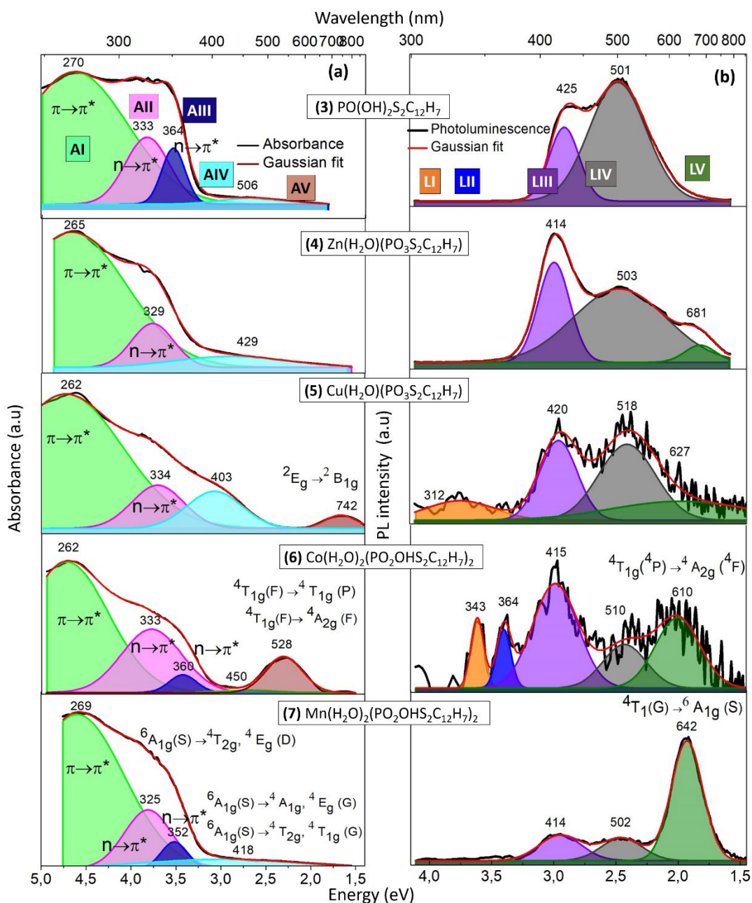
Figure 10: Absorbance (a) and Photoluminescence with excitation at 4.66eV (266 nm) (b) spectra of thianthrene phosphonic acid PO(OH) 2 S 2 C 12 H 7 (3) and hybrid compounds, Zn(H 2 O)(PO 3 S 2 C 12 H 7 ) (4), Cu(H 2 O)(PO 3 S 2 C 12 H 7 ) (5), Co(H 2 O) 2 (PO 2 OH-S 2 C 12 H 7 ) 2 (6) and Mn(H 2 O) 2 (PO 2 OH-S 2 C 12 H 7 ) 2 (7)] absorbance and emission peaks fitted by Gaussian functions.
