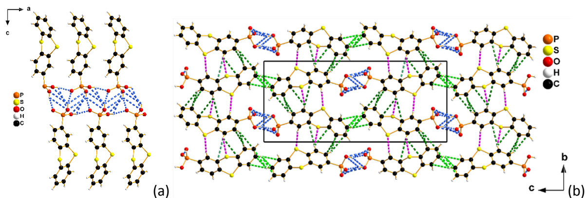
Figure 4 : (a) Zigzag network of hydrogen bonds, with \text{O}\cdots\text{H}-\text{O} distances ranging from 1.7999(17) Å to 3.2623(17) Å. (b) Structure of phosphonic acid of formula \text{PO}(\text{OH})_2\text{S}_2\text{C}_{12}\text{H}_7
