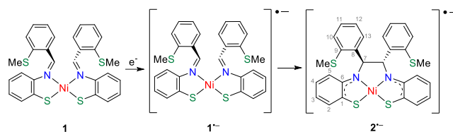
Scheme 3. Electron-triggered ligand dimerization of 1 to 2 - via unstable 1 - .
