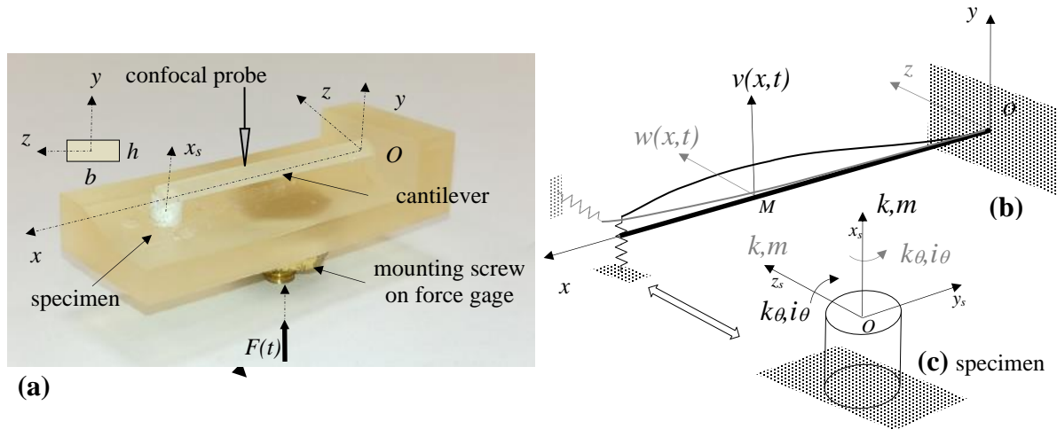
1 2 3 Figure 1 – (a) Experimental device: clamped beam simply supported on the elastic specimen with 4 (O,x,y,z) being the cantilever reference frame. (b) Diagram of the theoretical model: v(x,t) is the 5 cantilever transversal displacement in the vertical plane (O,x,y) and w(x,t) is the cantilever 6 transversal displacement in the horizontal plane (O,x,z) . (c) Specimen stiffness and mass properties: 7 k, k_\theta, m and i_\theta are involved into the dynamic vertical response (—) and k, k_\theta, m and i_\theta are involved 8 into the dynamic horizontal response (---). The excitation force is F(t) . 9 10
