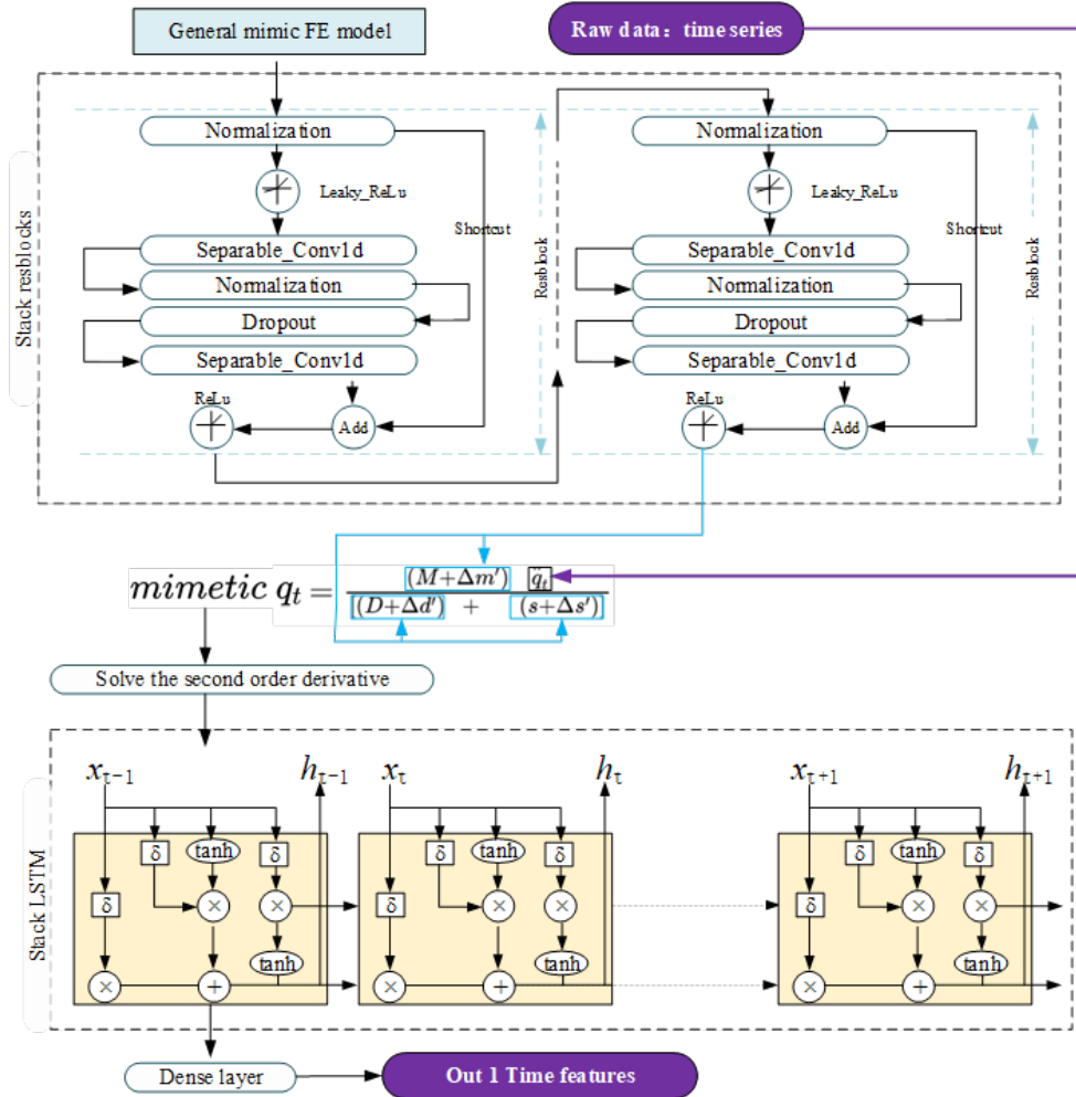
Figure 8: Structure of CNN-LSTM layer to mimic the FEM solution process
