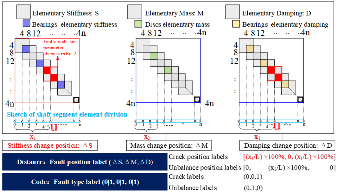
Figure 2: Relation between the matrices of the structural parameter, fault type, and fault location labels
