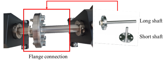
Figure 12: Schematic diagram of the shaft-cracking experiment.
