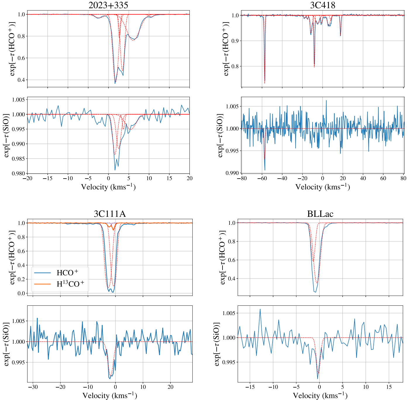
Figure 2. The \text{HCO}^+ (top) and SiO (bottom) absorption spectra ( e^{-\tau} ) in the direction of our eight background sources. Gaussian fits are shown as red dashed lines for both species. For 3C 111A, we also show the \text{H}^{13}\text{CO}^+ absorption spectra and Gaussian fits.
