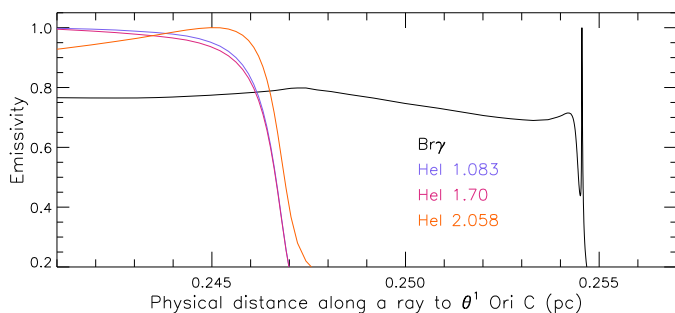
Fig. 13. Emissivity profile of selected transitions as a function of the physical distance along a ray from \theta^1 Ori C and perpendicular to the Bar given by a Cloudy model employing the physical parameters derived by Shaw et al. (2009) and Pellegrini et al. (2009). See Sect. 6.2 for details.
