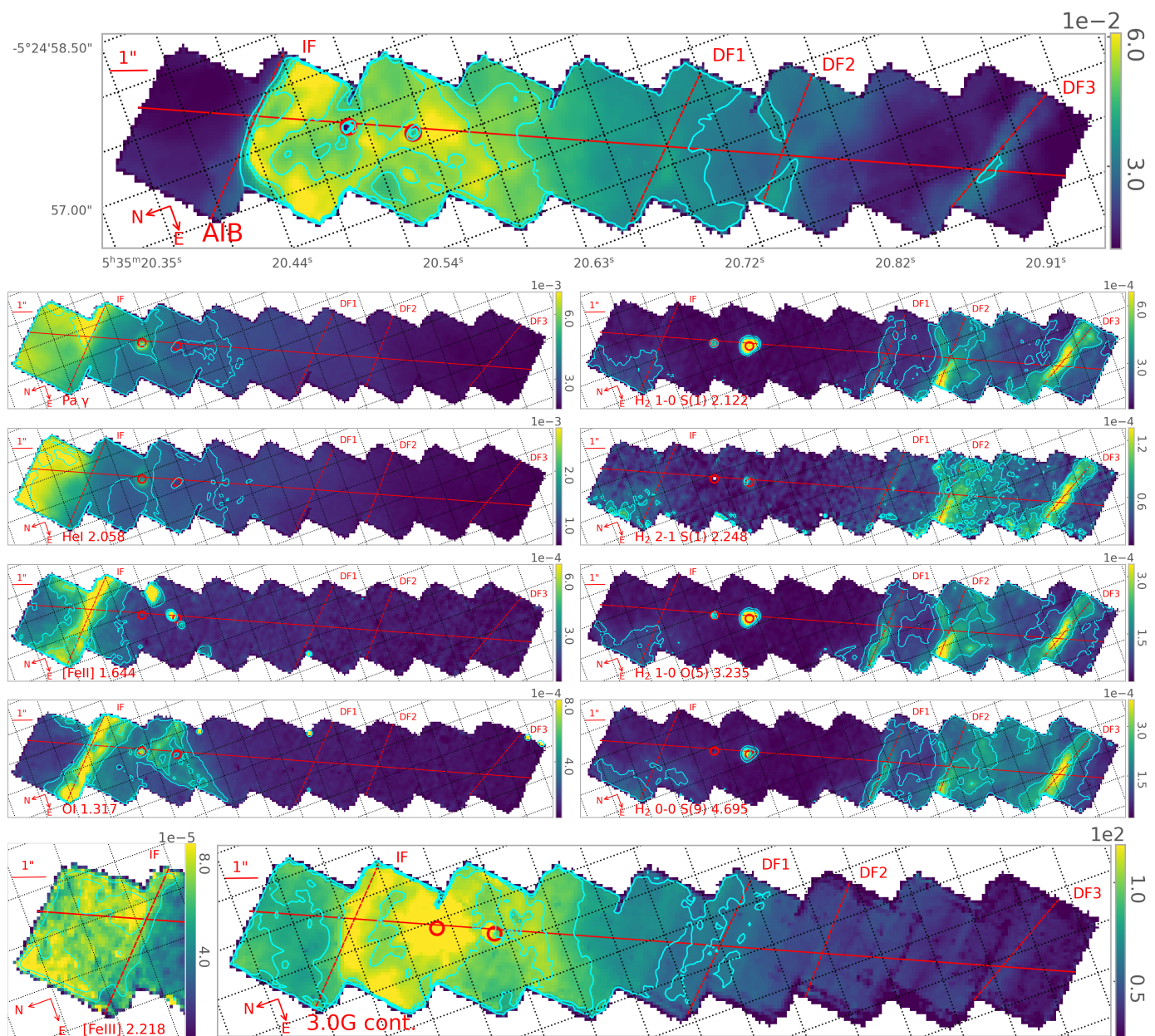
Fig. 7. The Bar as seen in selected transitions in units of \text{erg cm}^{-2} \text{s}^{-1} \text{sr}^{-1} . No extinction correction is applied. Starting at the top, we show an image of the total AIB emission (i.e. sum of all AIB components in the 3.2 - 3.7 \mu\text{m} range). Following that, (from top to bottom) we show Pa \gamma , He \text{I } 2.058 \mu\text{m} , [Fe \text{II} ] 1.644 \mu\text{m} , O \text{I } 1.317 \mu\text{m} , and [Fe \text{III} ] 3.22 \mu\text{m} in the left column and H _2 1-0 S(1), H _2 2-1 S(1), H _2 1-0 O(5), H _2 0-0 S(9), and the continuum from the Gaussian decomposition at 3 \mu\text{m} ( \text{MJy sr}^{-1} ) in the right column. We set the colour range from the bottom 0.5 % to the top 99.5 % intensity levels of the data for each map (across the entire NIRSspec mosaic), excluding values of zero, edge pixels, and the two proplyds (as well as the surrounding region of the proplyds for the continuum). White pixels inside the mosaic indicate values of zero reflecting issues with the data. The nearly horizontal red line indicates the NIRSspec cut and the nearly vertical red lines indicate from left to right the DFs (DF 3, DF 2, DF 1) and the IF. The two proplyds are indicated by the circles. Across the entire NIRSspec mosaic, contours show the 52, 75, and 90 % intensity levels of the data for AIB, 65, 80, 98 % intensity levels for Pa \gamma and He \text{I } 2.058 \mu\text{m} , 77.9, 90.2, 96 % intensity levels for O \text{I } 1.317 \mu\text{m} and [Fe \text{II} ] 1.644 \mu\text{m} , 87.7, 94.9 % intensity levels for [Fe \text{III} ] 2.218 \mu\text{m} , 60, 90, 98 % intensity levels for H _2 (excluding H _2 2-1 S(1), which uses 80, 90, 98 % intensity levels), and the 50, 68, 85 % intensity levels for the continuum at 3 \mu\text{m} . We note that a smoothing is applied to the [Fe \text{III} ] 2.218 \mu\text{m} contour levels.
