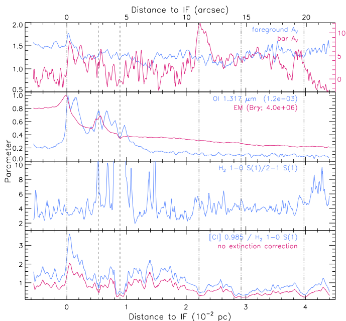
Fig. 11. Foreground and internal PDR extinction (top panel), O I 1.317 \mu m line flux and emission measure (second panel) and line flux ratios (lower two panels) as a function of distance to the IF (0.228 pc or 113.4'' from \theta^1 Ori C) along a cut crossing the NIRSpc mosaic (see Fig. 1). As the cut is not perpendicular to the IF and distances are given along the cut, a correction factor of \cos(19.58^\circ)=0.942 needs to be applied to obtain a perpendicular distance from the IF. Foreground extinction correction is applied to determine bar A_V ( A_{V_{bar}} ) and for the line intensities and ratios depicted in blue colour. The dash-dot-dot-dot vertical lines indicate the position of the IF, DF 1, DF 2, and DF 3 respectively from left to right. The dashed vertical lines indicated the location of the proplyds 203-504 (left) and 203-506 (right).
