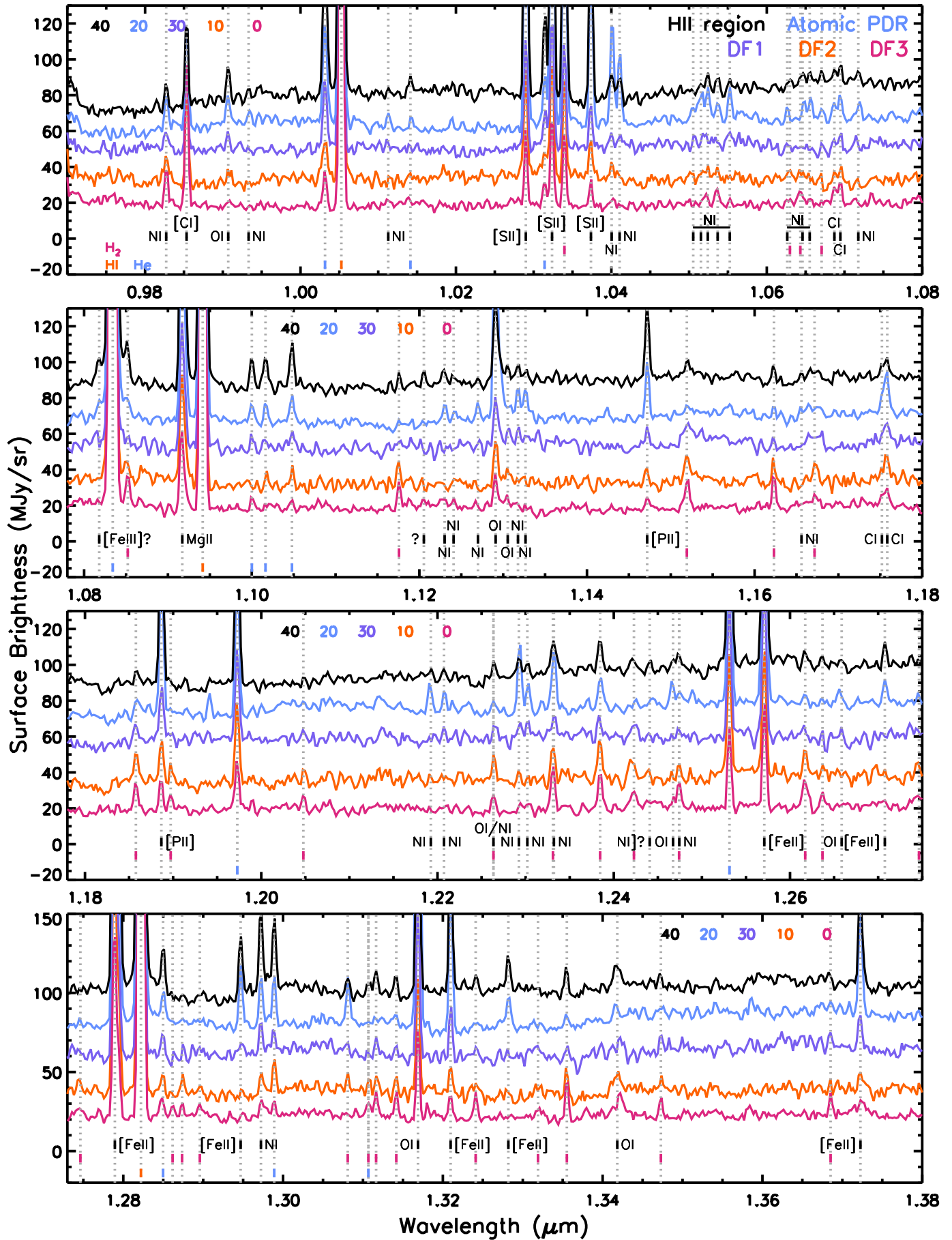
Fig. B.1. The spectral inventory of the five template spectra. Spectra are offset by the numbers given at the top of the panel. Areas susceptible to the wavelength gap are shown in light grey. The color coding is labeled in the top panel.
