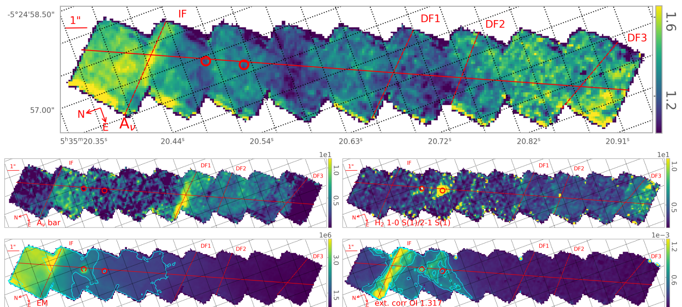
Fig. 10. Starting at the top, we show an image of the visual line-of-sight fore-ground extinction A_V (Sect. 6.1). Next, from left to right, we show the visual line-of-sight internal PDR extinction A_{V\text{bar}} and the \text{H}_2 1-0 S(1)/2-1 S(1) ratio. Lastly, we show the Emission Measure (EM; in units of \text{pc cm}^{-6} , Sect. 6.1) and the extinction corrected O I 1.317 \mu\text{m} (ext. corr. O I 1.317 \mu\text{m} ; in units of \text{erg cm}^{-2} \text{s}^{-1} \text{sr}^{-1} ), respectively. We set the color range from the bottom 0.5 % to the top 99.5 % of data for each map, excluding values of zero, edge pixels, and the two proplyds. White pixels inside the mosaic indicate values of zero reflecting issues with the data. The nearly horizontal red line indicates the NIRSpec cut and the nearly vertical red lines indicate from left to right the DFs (DF 3, DF 2, DF 1) and the IF. The two proplyds are indicated by the circles. Contours show the 55, 78, and 98 % of the data for EM, and 77.9, 90.2, and 96 for O I 1.317 \mu\text{m} .
