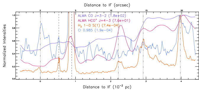
Fig. 20. Comparison of the NIRSpec \text{H}_2 1-0 S(1) and \text{C I} 0.985 \mu\text{m} observations (in \text{erg cm}^{-2} \text{s}^{-1} \text{sr}^{-1} ) with ALMA observation at 1'' resolution of the \text{HCO}^+ J=4-3 line integrated intensity (in \text{K km s}^{-1} ) and the \text{CO } J=3-2 line peak temperatures ( T_{\text{peak}} ) Goicoechea et al. (2016). Shown are normalised line intensities as a function of distance to the IF (0.228 pc or 113.4'' from \theta^1 Ori C) along a cut crossing the NIRSpec mosaic (see Fig. 1). As the cut is not perpendicular to the IF and distances are given along the cut, a correction factor of \cos(19.58^\circ)=0.942 needs to be applied to obtain a perpendicular distance from the IF. No extinction correction is applied. The dash-dot-dot-dot vertical lines indicate the position of the IF, DF 1, DF 2, and DF 3, respectively, from left to right. The dashed vertical lines indicated the location of the proplyds 203-504 (left) and 203-506 (right).
