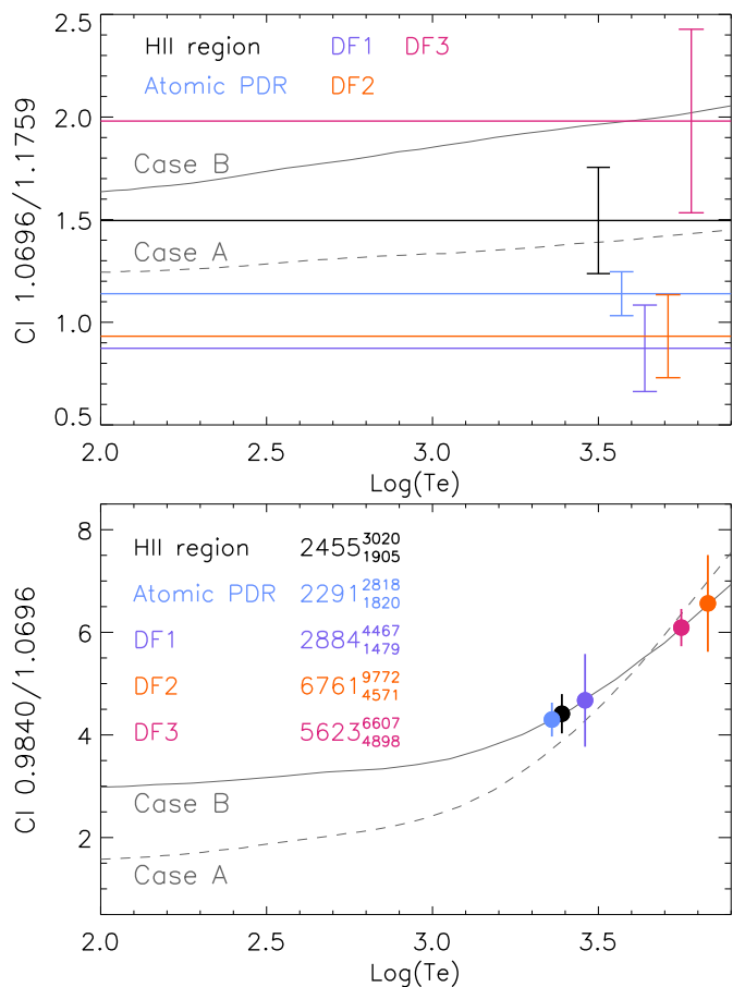
Fig. F.1. Comparison of extinction corrected C I line ratios with computed ratios taken from Walmsley et al. (2000) that are based on calculations of Escalante & Victor (1990) for both case A and case B recombination theory. Uncertainties on the observed ratios are given by vertical lines that are placed at the derived electron temperature (lower panel) or in the [3.5 – 3.8] x-range (top panel).
