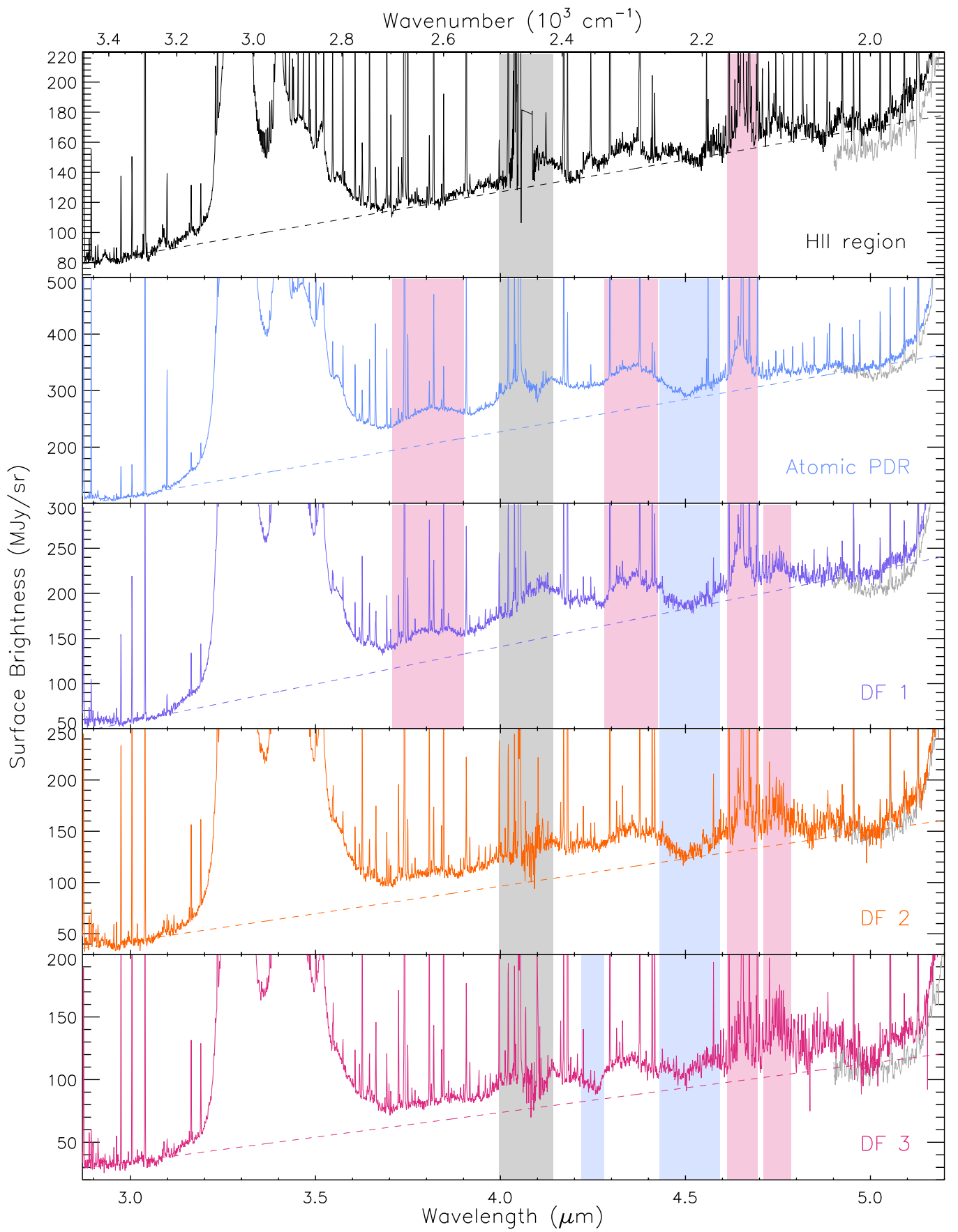
Fig. 6. Illustration of excess broad band emission between 3 – 5 \mu\text{m} . Close to the wavelength gap, fluxes are often unreliable (Sect. 3.2; indicated by the grey shaded area). The MIRI spectra are shown in light grey. The dashed lines show a linear continuum matched with the data near 2.98 and 4.99 \mu\text{m} . Red (blue) shaded boxes indicate tentative emission (absorption) bands. See Sect. 4 for a discussion.
