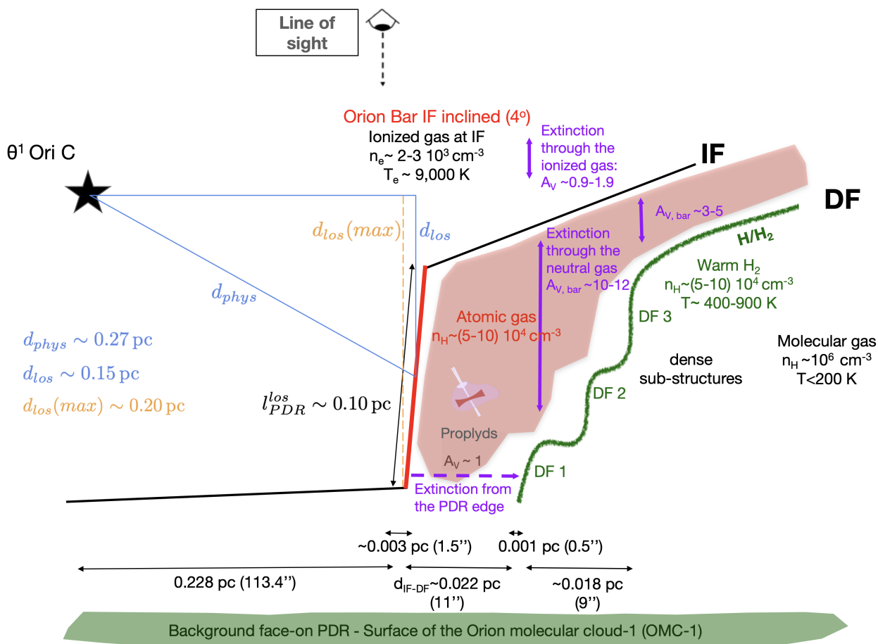
Fig. 14. Schematic overview of the Bar as inferred from JWST and other observations (e.g. Jansen et al. 1995; Wen & O’Dell 1995; O’Dell 2001; Pellegrini et al. 2009). It shows the main features discussed in this paper and Habart et al. (2023, based on NIRCам and MIRI imaging). Given the complexity of the PDR surface, parameters derived in this paper are specific for the NIRSpect mosaic. Note that for clarity, the dimensions perpendicular to the bar are not to scale; the true spatial scales are explicitly given in the annotations. In addition, the sketch does not include foreground material, that includes a layer of ionised gas O’Dell et al. (2020) and, closer to the observer, layers that are grouped together under the designation as the Veil (e.g., Rubin et al. 2011; Boersma et al. 2012; van der Werf et al. 2013; Pabst et al. 2019, 2020).
