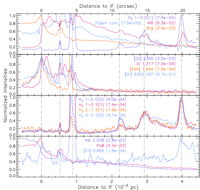
Fig. 9. Normalised line intensities as a function of distance to the IF (0.228 pc or 113.4'' from \theta^1 Ori C) along a cut crossing the NIRSpc mosaic (see also Figs. 1 and 7 for the location of the cut). As the cut is not perpendicular to the IF and distances are given along the cut, a correction factor of \cos(19.58^\circ)=0.942 needs to be applied to obtain a perpendicular distance from the IF. No extinction correction is applied. For reference, we show the extinction corrected [O I] 6300 Å emission observed by Weilbacher et al. (2015) and the [O I] 6300 Å emission observed by Bally et al. (2000) along the same cut. The dash-dot-dot-dot vertical lines indicate the position of the IF, DF 1, DF 2, and DF 3 respectively from left to right. The dashed vertical lines indicated the location of the proplyds 203-504 (left) and 203-506 (right). Units are \text{erg cm}^{-2} \text{s}^{-1} \text{sr}^{-1} except for the 3.0 \mu\text{m} continuum which is in MJy/sr.
