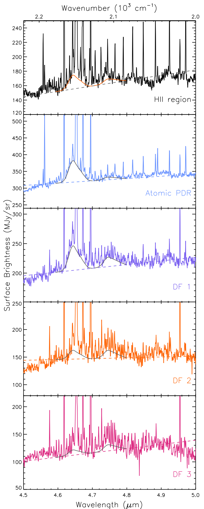
Fig. G.1. The tentative 4.644 and 4.746 \mu\text{m} dust features attributed to deuterated PAHs (Sect. 4). Local linear continua are shown by the dashed lines. The 4.646 and 4.746 \mu\text{m} bands are plotted on top of the continuum as a solid line. The same band profile for each feature is used for all templates. See Appendix G.2 for details.
