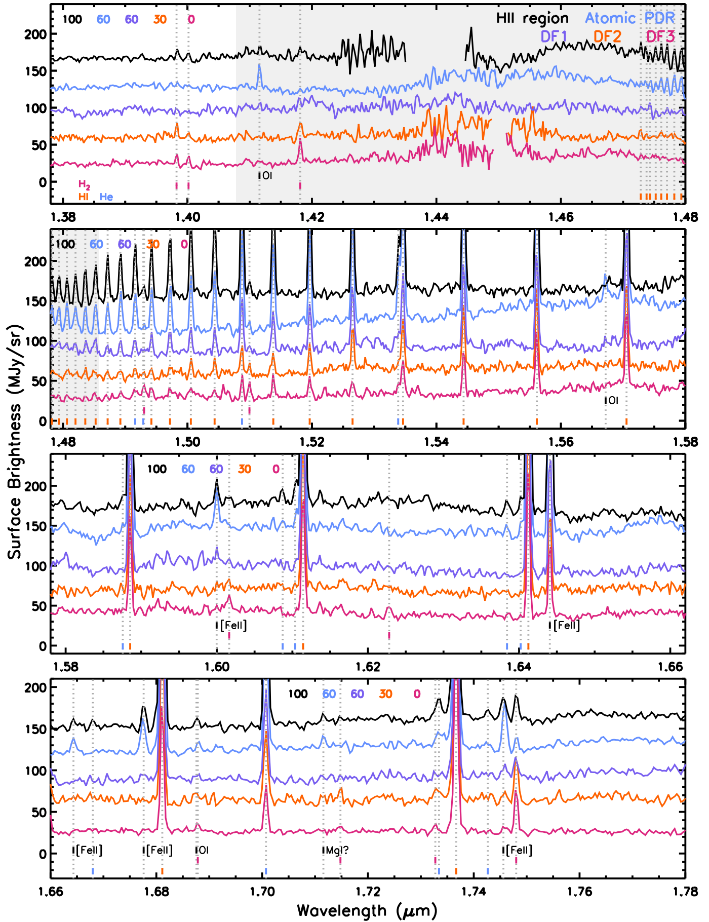
Fig. B.2. Fig. B.1 continued.
