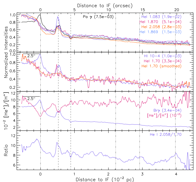
Fig. 12. Analysis of the He I and H I radial profiles as a function of distance to the IF (0.228 pc or 113.4'' from \theta^1 Ori C) along a cut crossing the NIRSpc mosaic (see Fig. 1). As the cut is not perpendicular to the IF and distances are given along the cut, a correction factor of \cos(19.58^\circ)=0.942 needs to be applied to obtain a perpendicular distance from the IF. Top two panels: Observed normalised line intensities of selected transitions. No extinction correction is applied. Units are in \text{erg cm}^{-2} \text{s}^{-1} \text{sr}^{-1} . Third panel: The [\text{He}^+]/[\text{H}^+] abundance. The normalised Br \gamma radial profile is shown for reference. Bottom panel: The He I 2.058/1.70 radial profile. The dash-dot-dot-dot vertical lines indicate the position of the IF, DF 1, DF 2, and DF 3, respectively, from left to right. The dashed vertical lines indicated the location of the proplyds 203-504 (left) and 203-506 (right).
