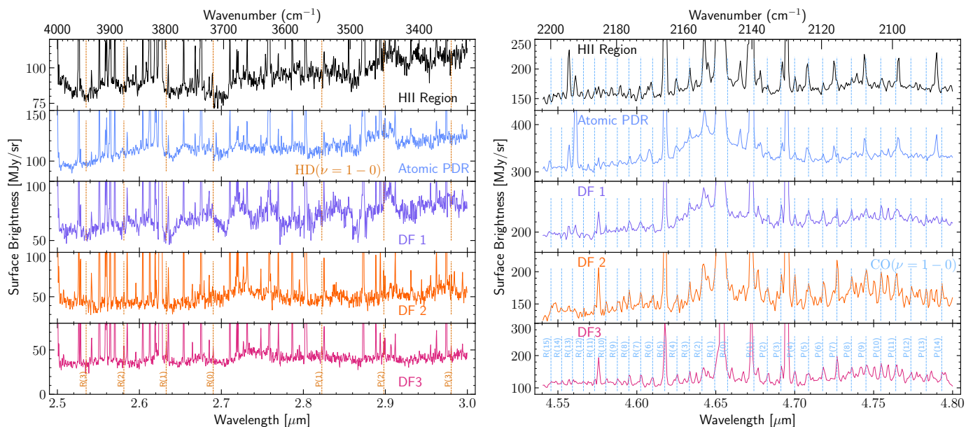
Fig. 3. Left: Detection of the HD \nu = 1 - 0 ro-vibrational lines at \sim 2.6 \mu\text{m} in the atomic PDR and molecular PDR. Right: Detection of the CO \nu = 1 - 0 band centered at 4.7 \mu\text{m} in the molecular PDR. For the CO \nu = 2 - 1 band detection, see Figs. B.7 and B.8.
