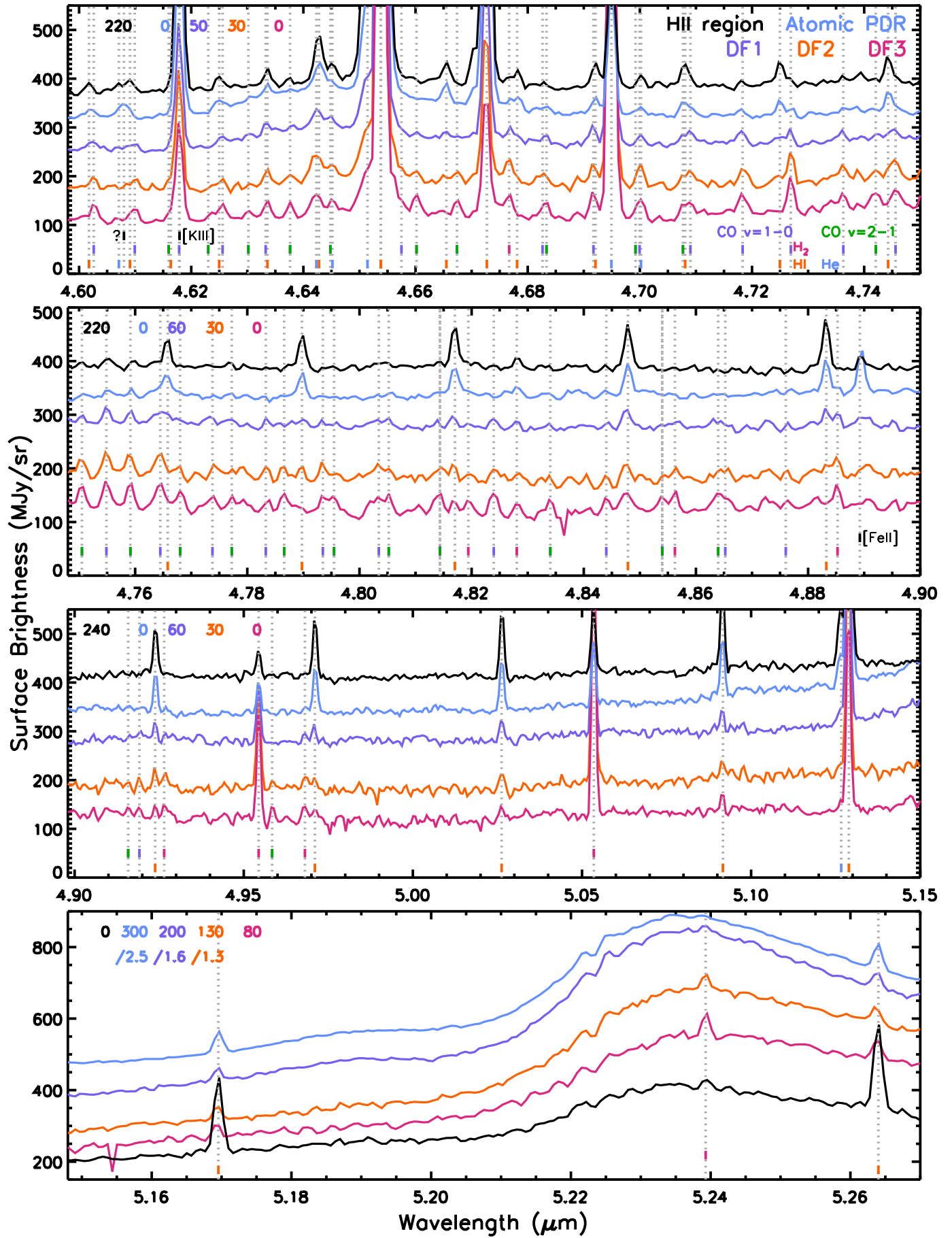
Fig. B.8. Fig. B.1 continued.
