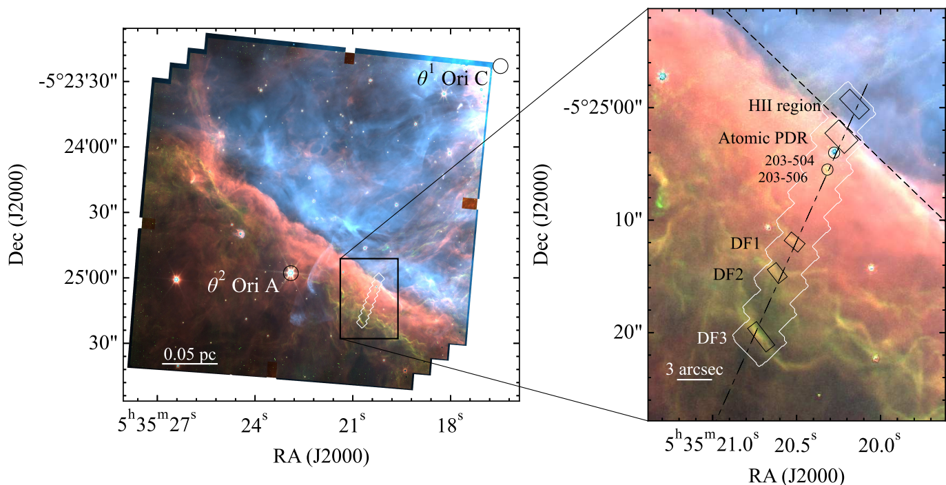
Fig. 1. Composite NIRCam image of the Bar showing the NIRSpect mosaic footprint (white boundary). The composite image is composed of F335M (AIB emission) in red, F470N-F480M ( H_2 emission) in green, and F187N (Paschen \alpha emission) in blue (Habart et al. 2023). Bright stars \theta^1 Ori C and \theta^2 Ori A are indicated with black circles in the left panel. In the right panel the five black boxes indicate the apertures used to extract our five template spectra. The dot-dashed line indicates the cut perpendicular to the Bar (position angle, PA, of 155.79^\circ ), while the dashed line indicates the position of the ionisation front in the NIRSpect FOV (PA= 46.21^\circ ). The protoplanetary disks 203-504 and 203-506 are indicated with black circles.
