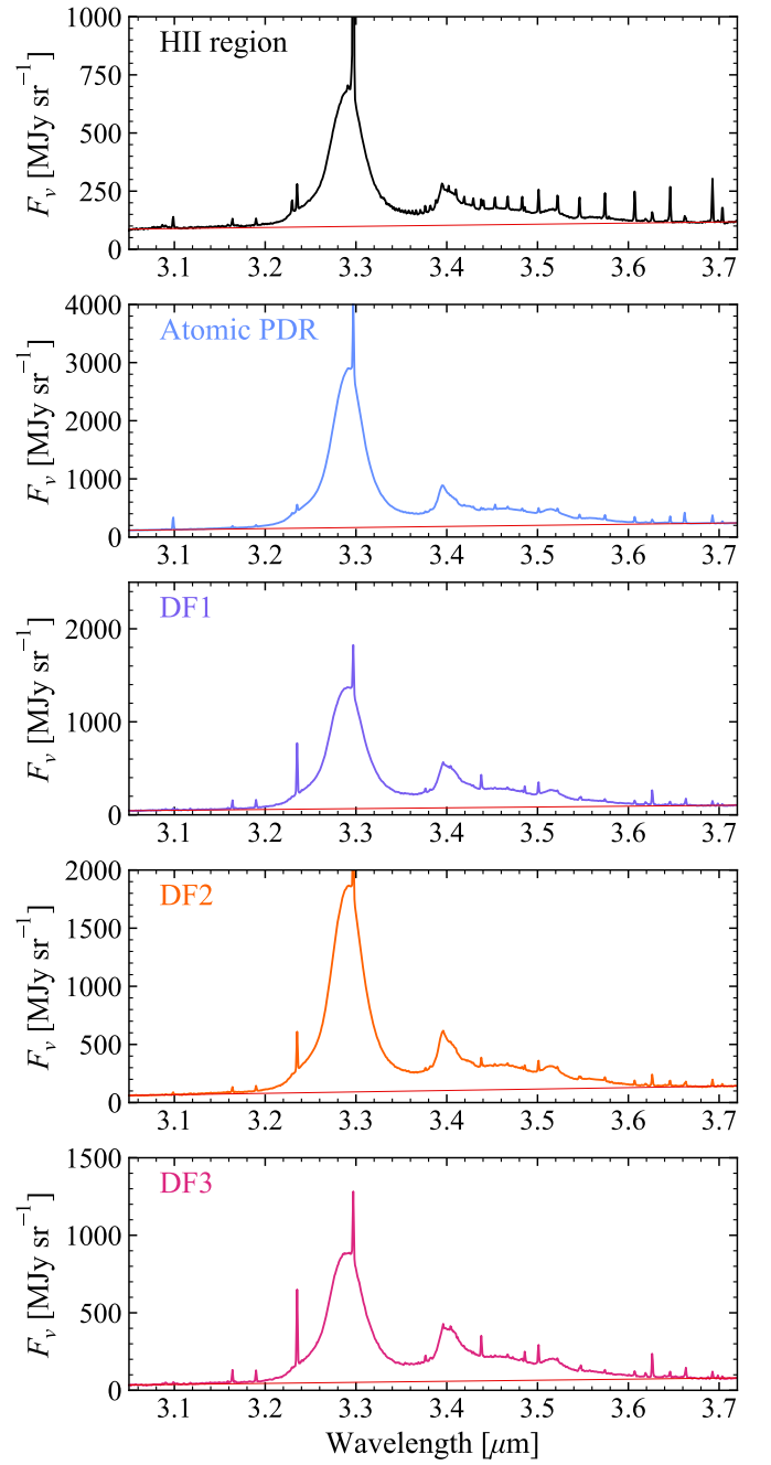
Fig. C.2. The NIRSspec template spectra (grating g395h, filter f290lp) from Peeters et al. (2023) along with their respective continua, zoomed in on the wavelength range that is relevant to the 3.3 \mu\text{m} AIB. See Sect. 2.3 and Appendix C for details.
