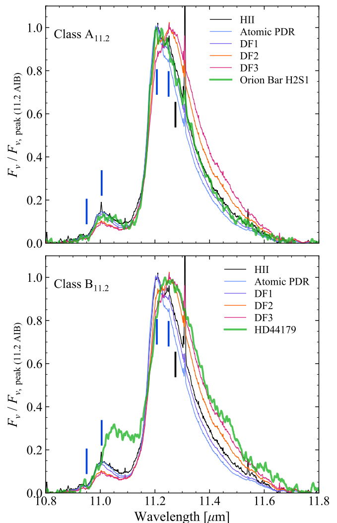
Fig. 6. Comparison of the 11.2\ \mu\text{m} profile in the five template spectra with a class A 11.2\ \mu\text{m} profile represented by the ISO-SWS spectrum of the Orion Bar H2S1 (van Dienenhoven et al. 2004, top panel) and a class B 11.2\ \mu\text{m} profile represented by the ISO-SWS spectrum of HD 44179 (van Dienenhoven et al. 2004, bottom panel).
