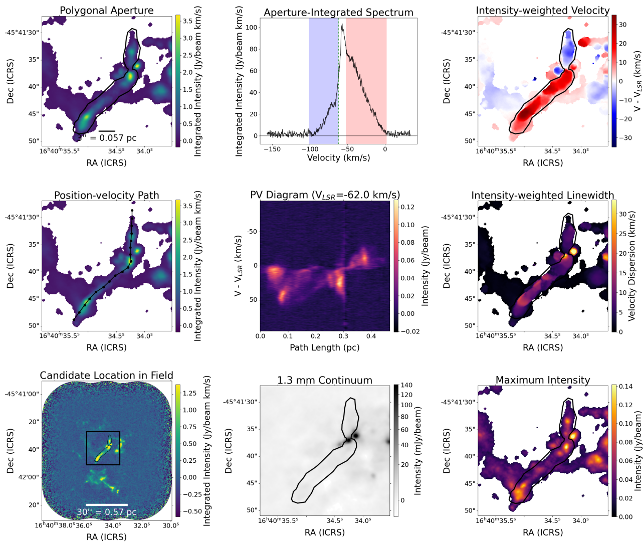
Figure 2. Same as in Figure 1, but for the asymmetric bipolar outflow Candidate #9 in field G338.93.
