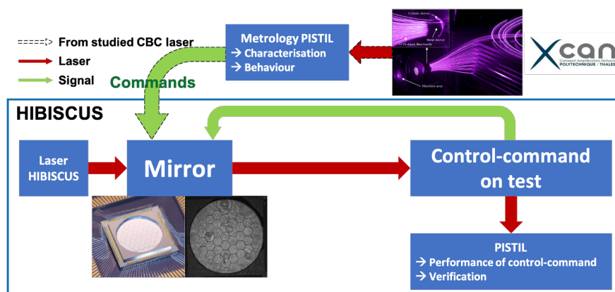
Figure 2. Schematic diagram of the HIBISCUS bench. The top part represents the phase drift measurements on the real laser by a metrology PISTIL. On the HIBISCUS bench, the behavioural command is sent to the mirror, illuminated by a working laser, to test the control system. Another PISTIL can be used for verification purposes.
