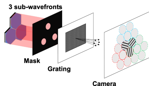
Figure 1. Schematic diagram of PISTIL: the beam, split by the mask, propagates through the grating in 3 pairs of \pm 1 orders before interfering at a given distance.
