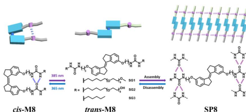
Figure 7. Schematic illustrations of the reversible photoisomerization and self-assembly of M8 . [155], Copyright 2021. Adapted with permission from the American Chemical Society.
