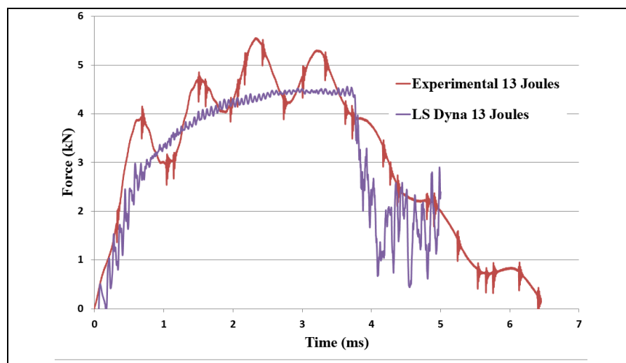
Fig . 12. Contact force history curves comparison
