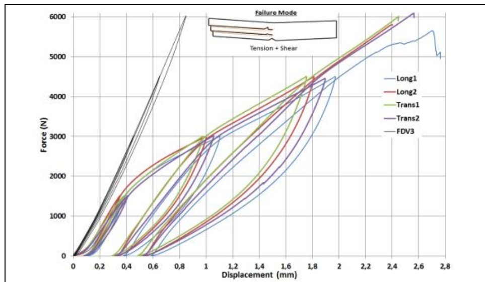
Fig. 4. Short 3 Point Bend for cyclic Test
