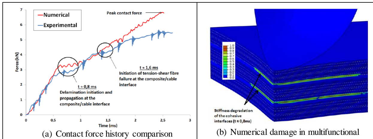
Fig .15. Damage influence take into account by the numerical model
