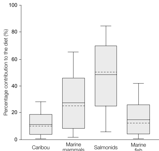
Fig. 6. Probability distribution of human diet composition, as estimated by FRUTS mixing model (adapted from McManus et al. 2018). Marine fish data taken from Byers et al. (2011).
