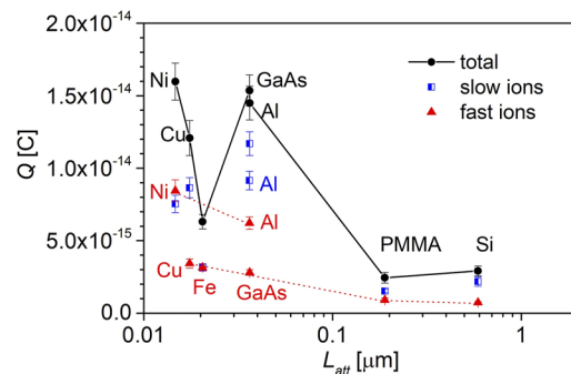
FIG. 12. Dependence of the charges Q_{\text{fast}} and Q_{\text{slow}} carried by fast and slow ions, respectively, and their sum on the attenuation length of 13.5 nm laser radiation in different targets. Attenuation lengths were calculated for all the target materials used using the Henke method. 36
