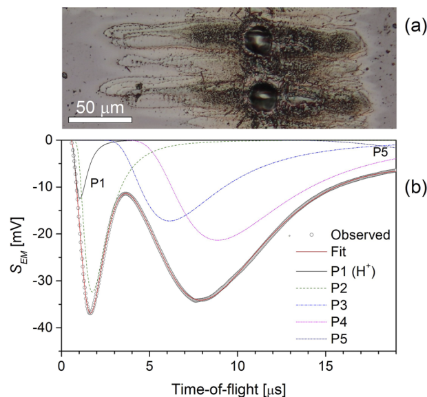
FIG. 9. (a) Ablative imprints in GaAs and (b) TOF spectrum of ions emitted by the GaAs target irradiated with energy 100 \mu\text{J} ( 2.7 \times 10^{13} \text{ W/cm}^2 ).
