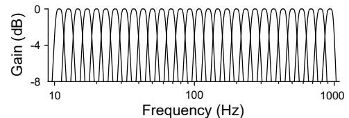
Fig. 3. Frequency response of the filter bank used to compute the power by frequency band of the vibration signals. The 30 filters are logarithmically spaced following Weber's law to match human perception.
