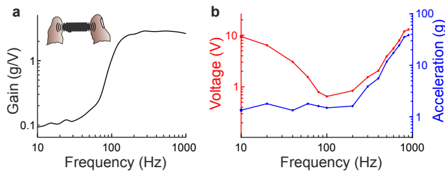
Fig. 1. a. Frequency response of the actuator held by two fingers, as in the experimental conditions. b. Iso-intensity vibration curve rendered by the actuator and felt with two fingers. The curves display the peak-to-peak voltage of the input signal (in red) and the peak-to-peak acceleration (in blue) corresponding to sine-waves at various frequencies that are perceived with the same intensity.
