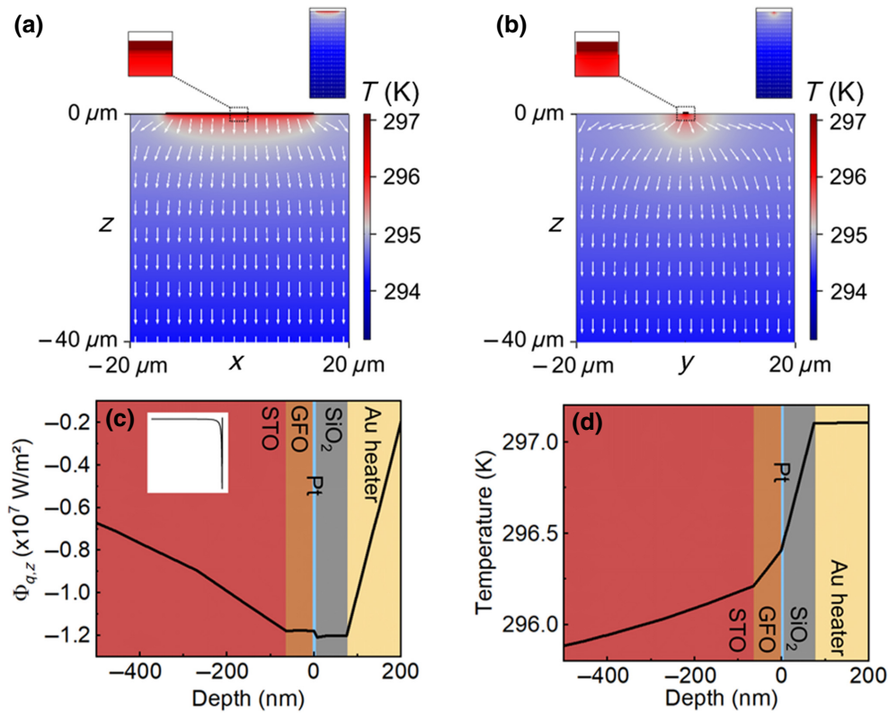
FIG. 4. Thermal simulation profile for the STO//GFO/Pt thermospin device. Calculated local temperature within the device that results from heating: (a) ( XZ ) cut plane and (b) ( OYZ ) cut plane. The insets show the same distribution near the device (top left) and at an expanded range through the whole system (top right). (c) z component of heat flux in the out-of-plane direction at the center of the device as calculated by the numerical method. The inset extends the range in depth including the substrate, showing that the heat flux close to the bottom of the substrate vanishes. (d) Temperature in the out-of-plane direction at the center of the device as calculated by the numerical method.
