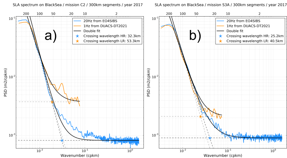
FIGURE 6 Mean SLA PSD over the Black Sea region, deduced from Cryosat-2 (A) and Sentinel-3A (B) measurements. The PSD obtained from 20Hz (resp. 1Hz) measurements is presented in blue (resp. orange). The spectral slope and noise level deduced from the PSD analysis are presented in dotted black lines, while theoretical spectrum, defined as the sum of the spectral slope and noise, are presented in thick black lines. The intersection between the spectral slope and noise level is symbolized by a blue (yellow) star for 20Hz (1Hz) measurements. It is representative of the SNR equal unity.
