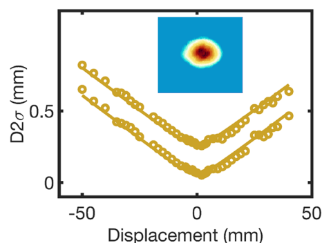
Figure 5. Beam profile. M^2 measurement of the HHG-mode signal at 1750 nm, with values of 1.3 and 1.4 along the major and minor axes, respectively. (The plots are vertically offset for clarity). The inset shows the unfocussed beam profile.
