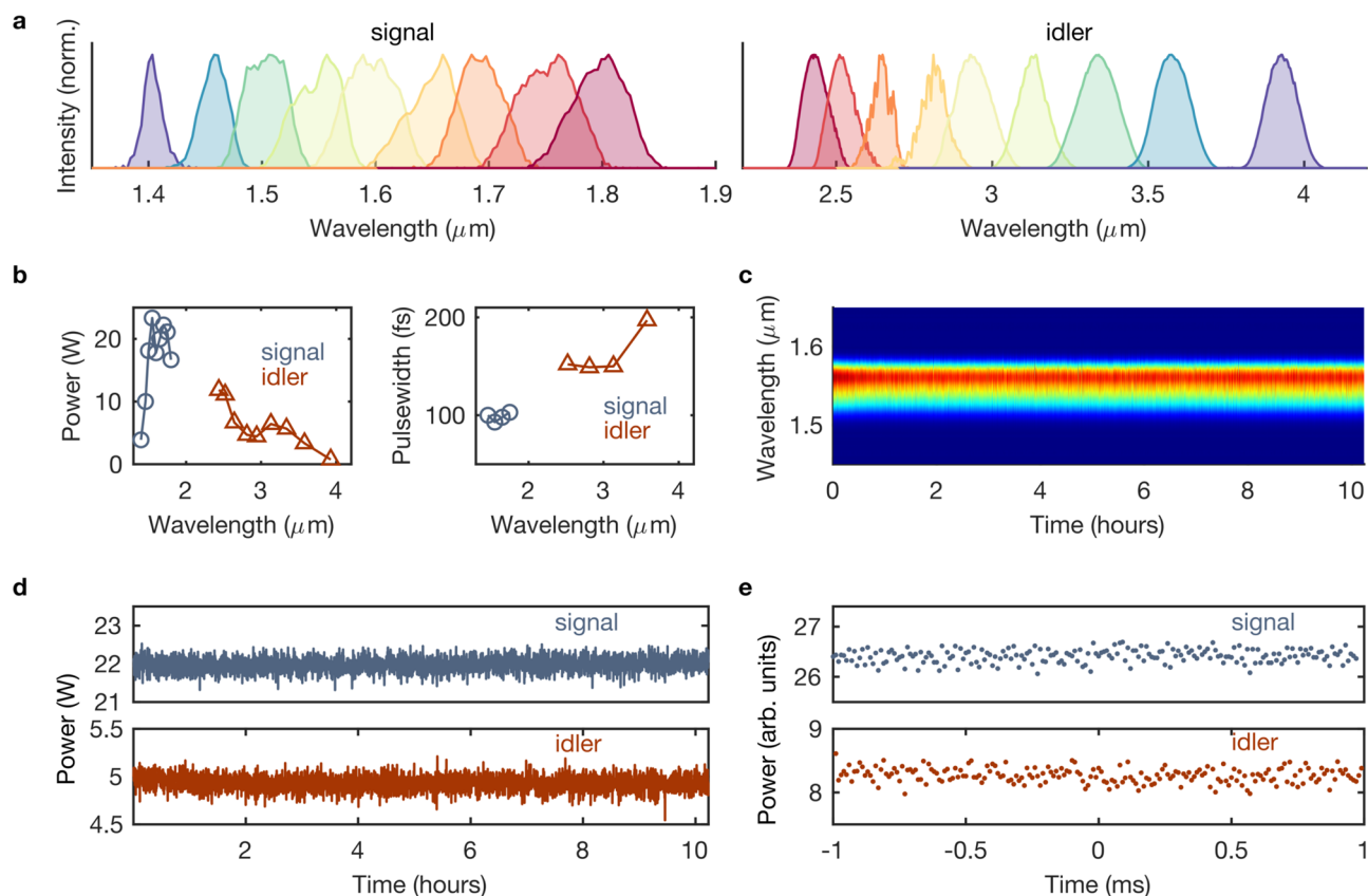
Figure 2. Tunable infrared spectroscopy mode. (a) Self-normalised signal and idler spectra. (b) Output power and measured pulse durations. (c) Spectral stability of the signal at 1.55 \mu\text{m} . (d) Power stability of the signal at 1.55 \mu\text{m} and the corresponding idler at 3.1 \mu\text{m} , with rms fluctuations of 0.8% and 1.5%, respectively, over 10 h. (e) Shot-to-shot stability, with rms fluctuations of 0.5% and 1.4% for the signal and idler, respectively, over 2 ms.
