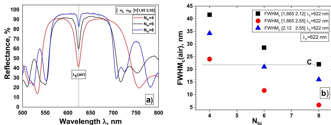
Figure 11. (a) Experimental reflectance spectra of microcavities with dependence of \text{fwhm}_c(\text{air}) on N_{\text{bilayer}} for structures with set [n_L, n_H] : [1.65, 2.12] , [1.65, 2.55] , [2.12, 2.55] and \lambda_c(\text{air}) = 622 nm and (b) dependence of \text{fwhm}_c(\text{air}) on N_{\text{bilayer}} for structures with set [n_L, n_H] : [1.65, 2.12] , [1.65, 2.55] , [2.12, 2.55] .
