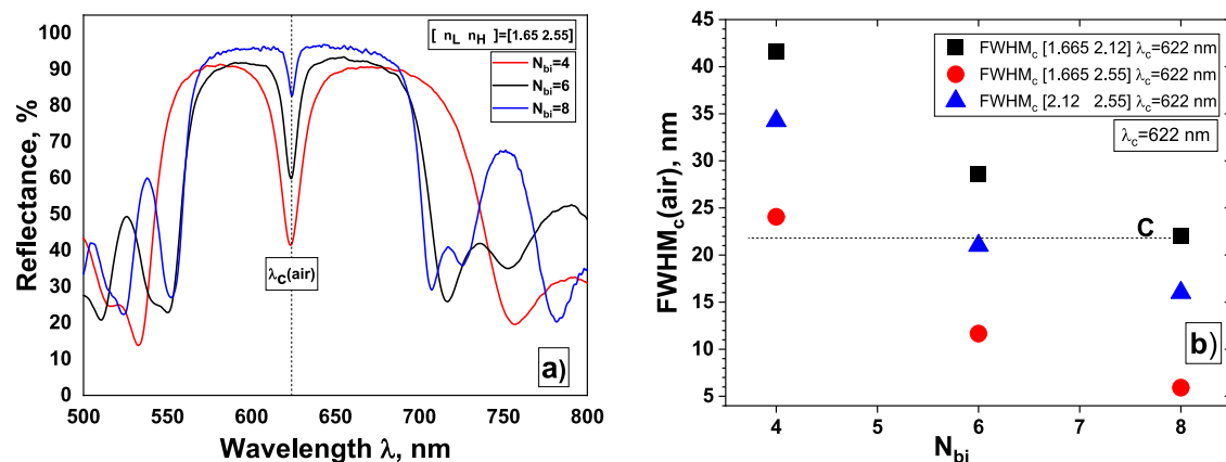
Figure 11. (a) Experimental reflectance spectra of microcavities with [n_L, n_H] = [1.65, 2.55] for N_{\text{bilayer}} = 4, 6, 8 and \lambda_c(\text{air}) = 622 nm and (b) dependence of \text{fwhm}_c(\text{air}) on N_{\text{bilayer}} for structures with set [n_L, n_H]: [1.65, 2.12], [1.65, 2.55], [2.12, 2.55] .
