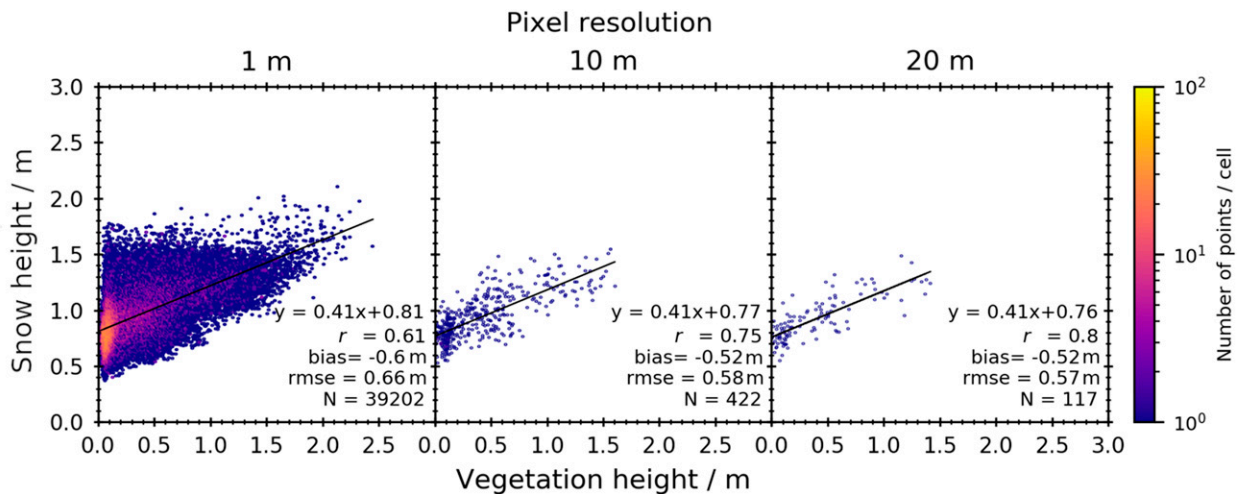
FIG. 8. Scatterplots of the relationship between vegetation height and snow height at the North site for pixel sizes of 1, 10, and 20 m. Owing to the large number of data points, the scatterplot was represented as hexbins colored by the number of data points contained within each bin. In this plot, each hexbin represents 1.5 \text{ m} \times 1.5 \text{ cm} . For all correlations, p values are <0.001 .
