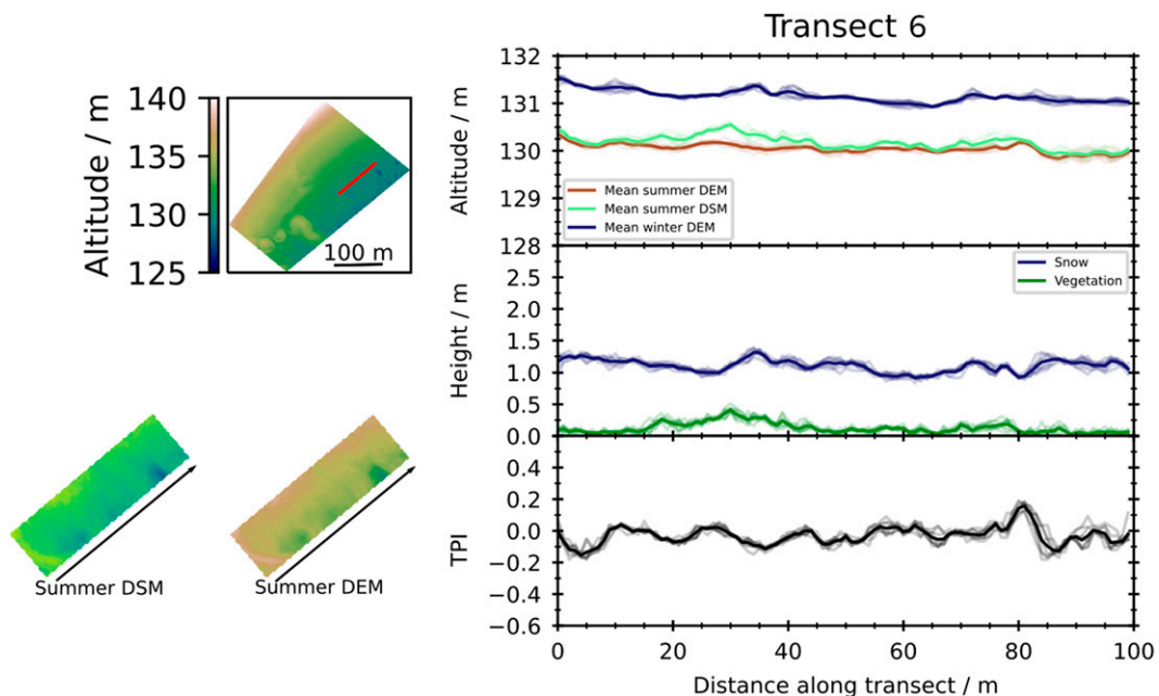
FIG. 19. Transect 6 in South site, as in Fig. 17. The start point of the averaged eight parallel transects is 56.55948^\circ , -76.47983^\circ (WGS84). The direction drawn is from west-southwest to east-northeast ( 50^\circ ).
