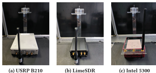
Figure 14: Two SDR devices and MiniPC with Intel 5300 WiFi card for conventional RF sensing.
