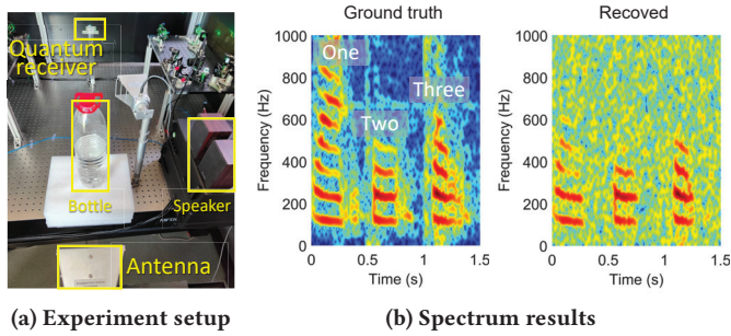
(a) Experiment setup (b) Spectrum results Figure 25: Sense subtle micrometer-level vibration induced by speaker to recover words (i.e., one, two and three).
