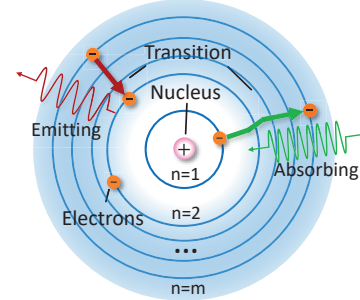
Figure 3: Illustration of atom structure and electron transition.
