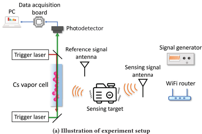
Figure 13: Experiment setup.
