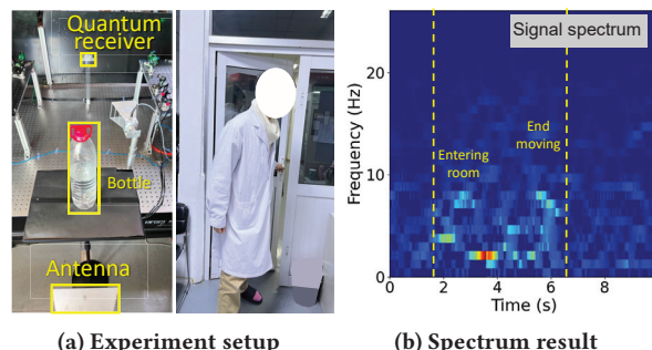
(a) Experiment setup (b) Spectrum result Figure 26: Sense object' micrometer-level subtle vibration induced by human walking.
