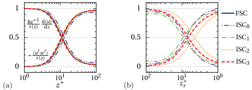
Fig. 2 Behavior of viscous and Reynolds stress (both normalized by the total mean shear stress) as a function of the wall-normal coordinate. Panel a : Situation near the bottom wall, as a function of z^+ . Panel b : situation near the surface, as a function of z_s^+ . Case FSC is not computed at the surface, and therefore, it is plotted only in panel (a)
