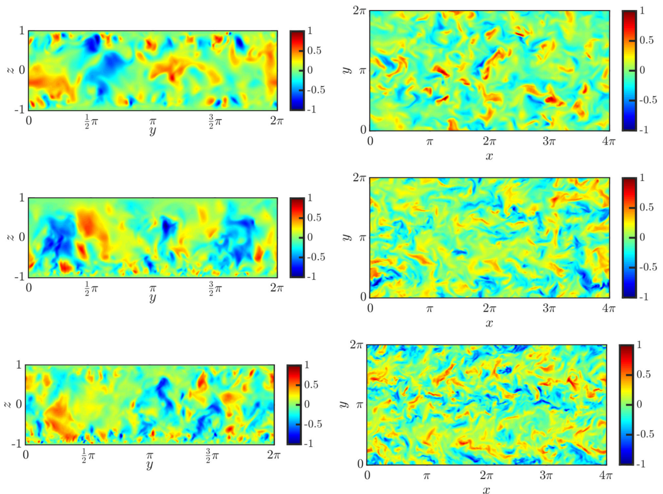
Fig. 12 Left column: Instantaneous vertical velocity w normalized by \max_{y,z}|w| in a transversal plane y - z . Right column: Instantaneous vertical velocity w normalized by \max_{x,y}|w| at the center of the channel, i.e., in the horizontal plane z = 0 . Top panels, ISC 0 ; Central panels, FSC; Bottom panels, ISC 3
