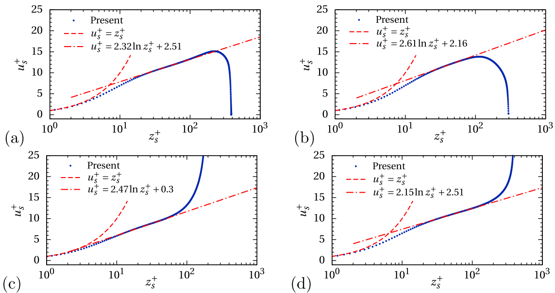
Fig. 16 Mean velocity profile u_s^+ computed from the surface boundary for the different ISC cases at Re = 180 : a ISC0, b ISC1, c ISC2, d ISC3. The behavior of the law of the wall is also shown for comparison (with parameters adjusted to fit to our data)
