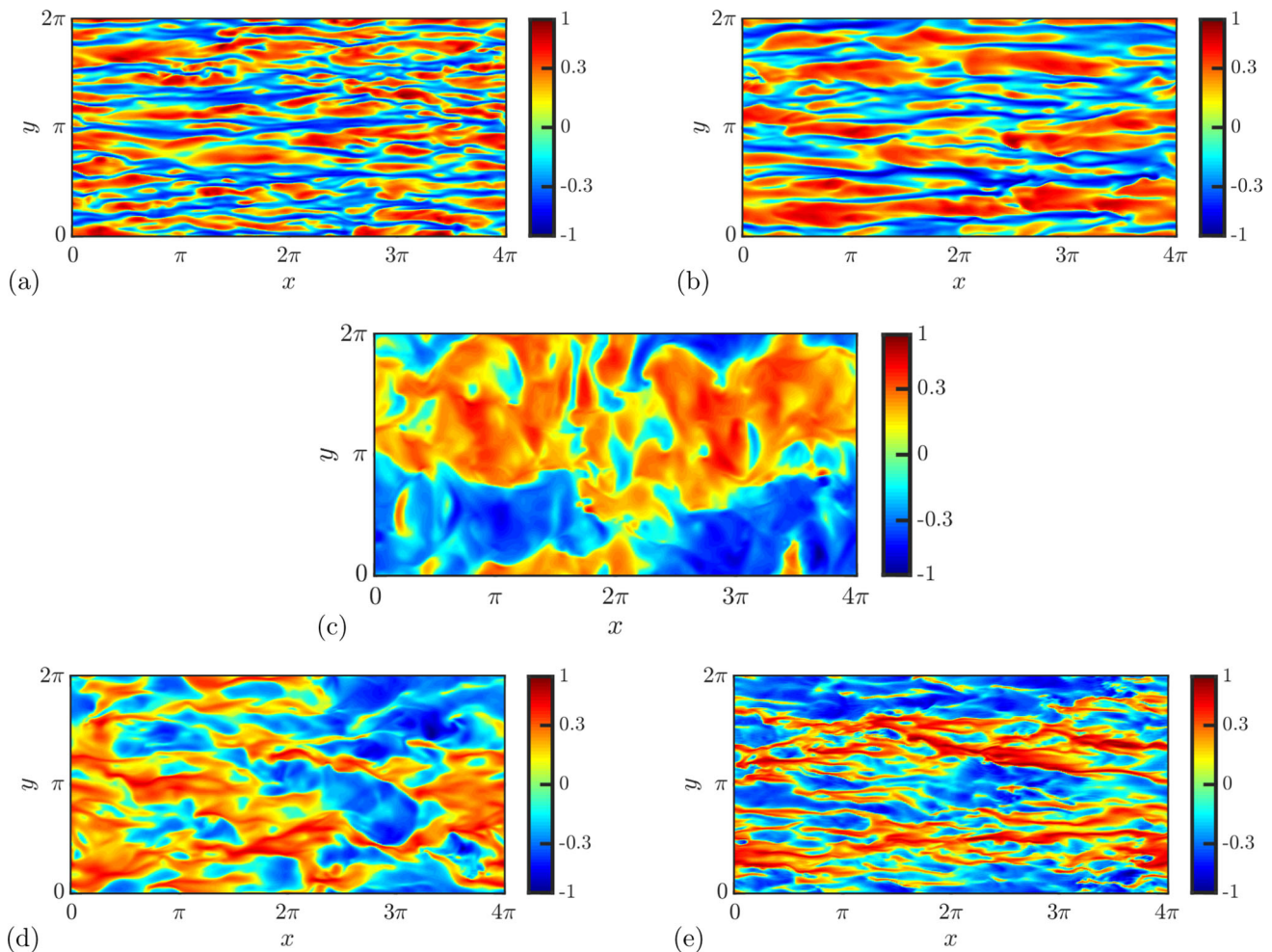
Fig. 20 Fluctuation u' of the instantaneous streamwise velocity, normalized by \max_{x,y} |u'| , at the horizontal plane z_3^+ = 5 located near the surface (except for the case FSC, for which the plot is located at \frac{1-z}{\delta_v} = 5 ). Instantaneous fields are taken at one representative time inside the statistically steady regime for a ISC 0 ; b ISC 01 ; c FSC; d ISC 2 ; e ISC 3 . Color bar is presented in quadratic scale
