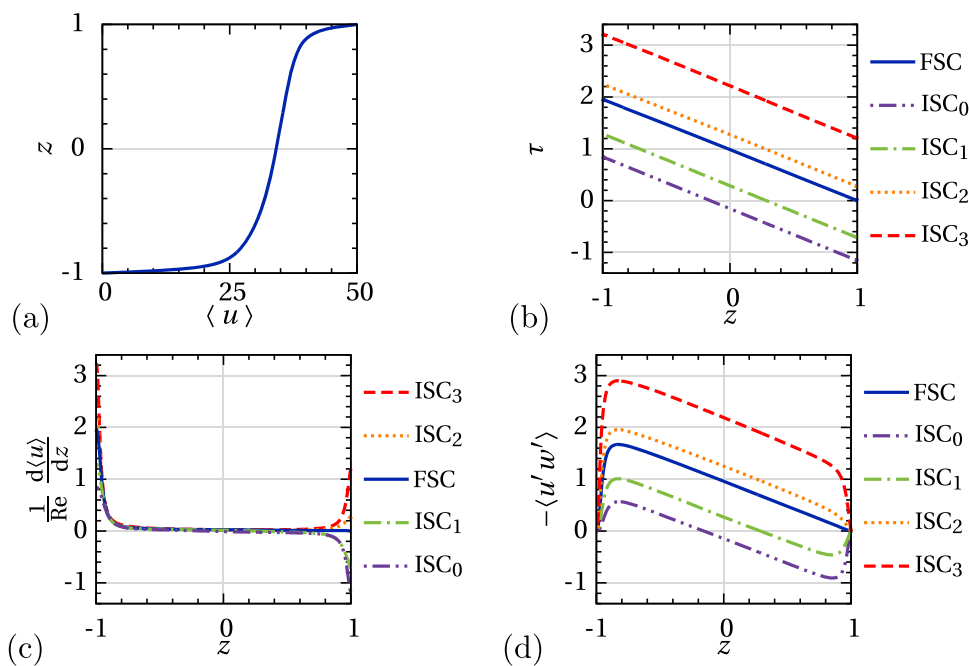
Fig. 14 a Mean streamwise velocity profile \langle u \rangle ; b mean shear stress \tau ; and its decomposition in viscous (c) and Reynolds stresses (d) . All cases are shown
