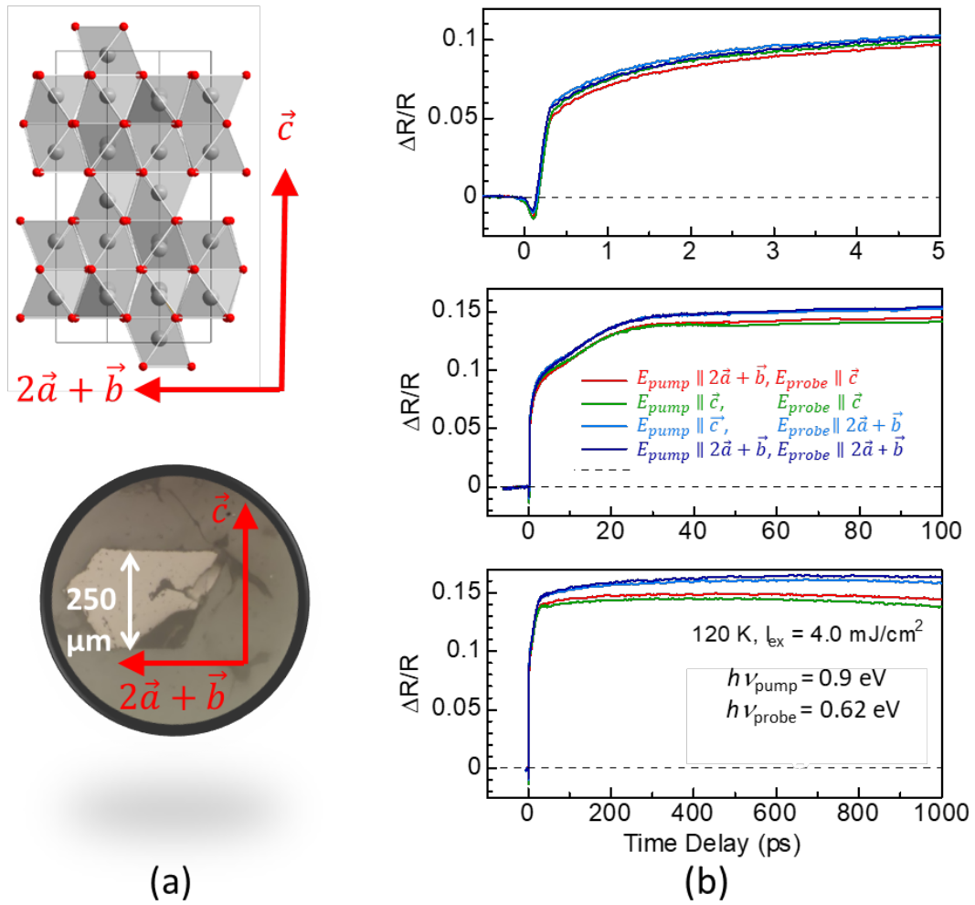
Extended data Fig.2 | Effect of single crystal orientation and pump/probe laser polarization on time-resolved reflectivity in the AFI state of V_2O_3 . In Fig.2 of the main article, we unveil a weaker photoinduced response of the single crystal with respect to thin film. In order to check if it results from an anisotropic response of V_2O_3 , we have performed polarization dependent tr-reflectivity after a proper orientation of a V_2O_3 single crystal by XRD and a polishing to reveal a surface suitable for tr-reflectivity. (a) optical image of the V_2O_3 crystal used for tr-reflectivity, with a surface defined by the the directions \vec{c} and 2\vec{a} + \vec{b} . (b) time-resolved reflectivity performed with polarization directions of the pump and the probe aligned along the \vec{c} and 2\vec{a} + \vec{b} directions after photoexcitation at 4 \text{ mJ}\cdot\text{cm}^{-2} at 120 K. Overall, the polarization effect is very weak and is hence not the cause of the weaker photoinduced response of the crystal shown in Fig.2 of the main text.
