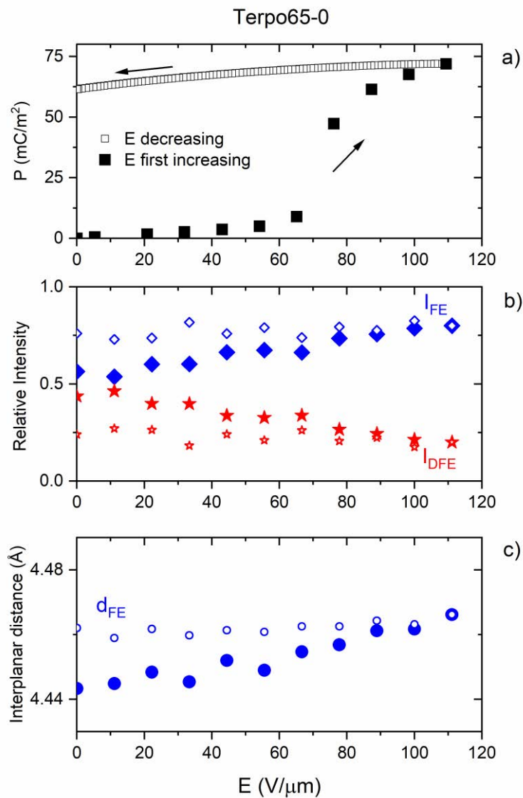
Figure 4: Structural evolution of the Terpo65-0 actuators under an electric field ( E ): first, E was gradually increased up to 110 V/\mu m , followed by a decrease back to 0 V/\mu m . a) Polarization, b) relative intensity of the DFE and FE Bragg peaks, and c) interplanar distance d_{FE} = d_{200}/d_{110} of the FE phase.
