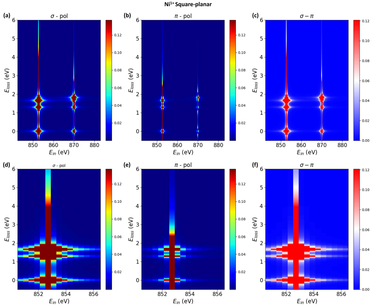
Figure S15: Calculated RIXS map at Ni-L edge of Ni 1+ Square-planar sites by Quany [6]. (a) Results for \sigma polarization, (b) \pi polarization, (c) Difference of both polarization ( \sigma - \pi ). (d-f) The magnified map at the Ni-L 3 edge. It has been obtained using D_q = 0.13 eV, \Delta_t = 0.10 eV, \Delta_s = 0.30 eV for the crystal-field parameters. It gives the following orbital energetic hierarchy : E_{x^2-y^2}(b1g) = 0 eV (reference) ; E_{xy}(b2g) = -1.30 eV ; E_{z^2-r^2}(a1g) = -1.70 eV ; E_{xz/yz}(eg) = -1.70 eV.
