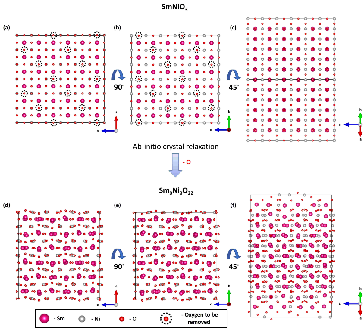
Figure S6: Ab-initio crystal structure relaxation of a 6 \times 6 \times 6 cubic supercell of \text{SmNiO}_3 with (303)_{pc} and (033)_{pc} oxygen vacancies, resulting in the \text{SmNiO}_{2.44} ( \text{Sm}_9\text{Ni}_9\text{O}_{22} ) structure. (a-c) The initial 6 \times 6 \times 6 supercell of cubic \text{SmNiO}_3 ( a = 3.79 \text{ \AA} ), along the (a) 0^\circ , (b) 90^\circ , and (c) 135^\circ projections. Note that the oxygen vacancies to be induced are indicated in (a) and (b), but they are not indicated along the 135^\circ projection in (c) due to overlap with other oxygen atoms. (d-f) The relaxed tetragonal structure along the (a) 0^\circ , (b) 90^\circ , and (c) 135^\circ projections. The in-plane parameters ( a = b = 3.79 \text{ \AA} ) are kept the same, while the out-of-plane parameter is reduced ( c = 3.63 \text{ \AA} ).
