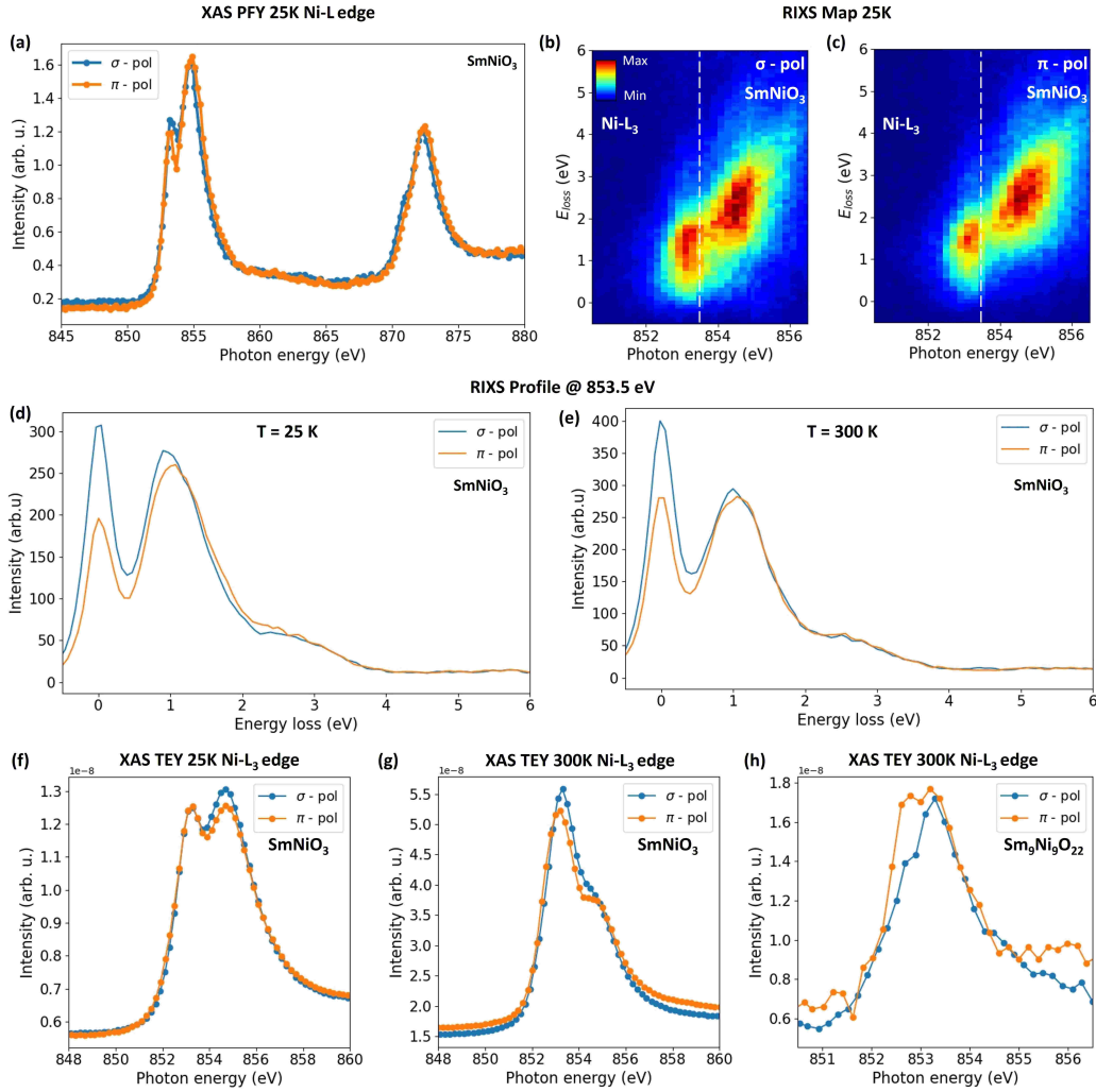
Figure S7: RIXS and XAS of SmNiO 3 and Sm 9 Ni 9 O 22 . (a) Partial fluorescence yield (PFY) XAS spectra at Ni - L edge of SmNiO 3 in two incident photon polarizations at 25K. (b & c) The corresponding RIXS maps at Ni - L 3 of SmNiO 3 in (b) \sigma polarization and (c) \pi polarization. (d & e) Temperature dependent variations in RIXS XLD profile from both polarizations in SmNiO 3 at 853.5 eV for (d) T = 25 K and (e) T = 300 K. (f & g) Total electron yield (TEY) XAS spectra at Ni - L 3 edge of SmNiO 3 for two incident polarizations at (f) T = 25 K and (g) T = 300 K. (f) TEY XAS spectra at Ni - L 3 edge of Sm 9 Ni 9 O 22 for two incident polarizations at 300 K. The XAS spectra in PFY and TEY mode are identical, as depicted here for SmNiO 3 . The TEY spectra of SmNiO 3 at 300K and 25K shows the metal-to-insulator transition, while the spectra of Sm 9 Ni 9 O 22 stays the same at 25K and 300K. Only TEY of the Ni-L are probed at 25K and 300K but they are very similar as the one reported by Bisogni et al. [1] showing that part of the thin film, certainly close to the surface is entering in the MIT coexistence. At RT, indeed the peak separation is getting smaller, and the width is changing very similarly as what they report by TEY in the case of NdNiO 3 . RIXS probes more bulk and hence shows weaker differences. Nevertheless, a small shift to higher energy is seen at \approx 1 eV energy loss measured at an excitation energy of 853.5 eV. It shows, at least, a partial charge disproportion when compared to the RIXS reported by Bisogni et al. [1].
