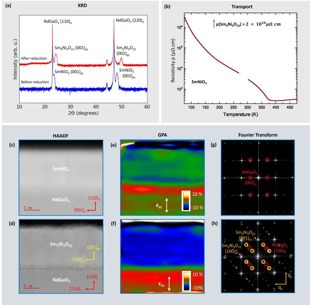
Fig. 1 Structural and transport comparison of SmNiO 3 with Sm 9 Ni 9 O 22 by XRD, HAADF-STEM imaging, GPA, and FT. (a) XRD comparison of both. The 001 and 002 peaks for SmNiO 3 occur at lower 2\theta values compared to the 001 and 002 peaks of Sm 9 Ni 9 O 22 , indicating an out-of-plane compression of the pseudocubic (pc) unit cell upon reduction. (b) Transport measurement of parent SmNiO 3 in increasing and decreasing temperatures. The resistivity curve of Sm 9 Ni 9 O 22 is not included in the plot since it was significantly higher, and is beyond the detection range of the equipment ( > 2 \times 10^{10} \mu\Omega.cm ). (c) HAADF-STEM image of SmNiO 3 thin film. (d) HAADF-STEM image of Sm 9 Ni 9 O 22 thin film, showing in good contrast the stripes coinciding with the (303) pc direction. (e & f) Maps of the o-o-p strain by GPA in (e) SmNiO 3 and (f) Sm 9 Ni 9 O 22 . Both samples show uniform o-o-p compression. The Sm 9 Ni 9 O 22 exhibits a more negative \epsilon_{zz} compared to SmNiO 3 , corresponding to a lower o-o-p parameter. (g & h) The corresponding FT of the HAADF image of (g) SmNiO 3 , (h) Sm 9 Ni 9 O 22 . The NGO substrate is indexed with an orthorhombic unit cell and the super-structure spots associated to the tilt pattern of the NGO are circled in red. The super-structure spots associated to the (303) pc stripes in Sm 9 Ni 9 O 22 are circled in yellow and are indexed within a pseudo-cubic unit cell.
