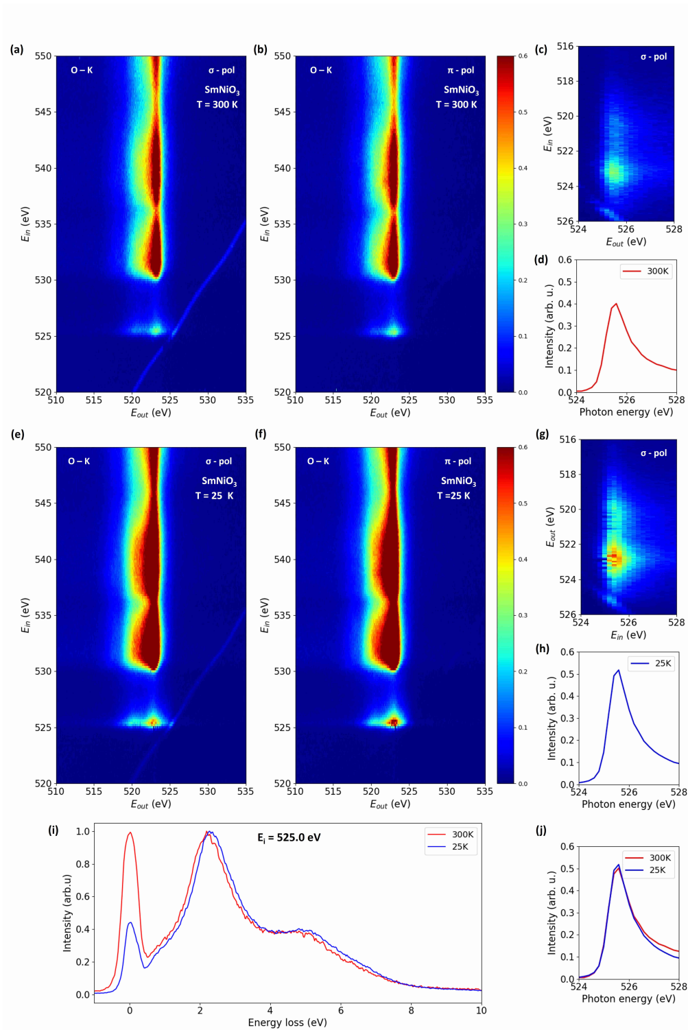
Figure S10: RIXS Map and XAS of O-K edge of SmNiO 3 showing a temperature dependent electronic transition. (a-d) Measurements at 300K. (a,b) RIXS map in incident ( E_{in} ) and detected ( E_{out} ) photon energy scales for (a) \sigma and (b) \pi incident photon polarisations, (c) A magnified RIXS map of a selected region in (a), (d) The XAS PFY plot of the O-K pre-edge, combining both polarisations. (e-h) Measurements at 25K. (e,f) RIXS map in incident ( E_{in} ) and detected ( E_{out} ) photon energy scales for (e) \sigma and (f) \pi incident photon polarisations, (g) A magnified RIXS map of a selected region in (e), (h) The XAS PFY plot of the O-K pre-edge, combining both polarisations. (i) Comparing the RIXS line profile at an incident photon energy of 525.0 eV for temperatures 300K and 25K, showing a blue shift at 300K. (j) The normalized-maxima-aligned pre-edge of O-K, for both temperatures. It shows a wider pre-edge at 300K.
