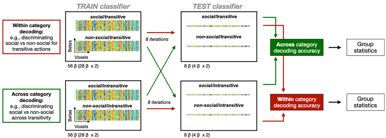
Figure 5. Schematic representation of the MVPA. A parameter ( \beta ) estimate was first extracted for each trial using a GLM. The SVM classification was performed using a leave-one-out cross-validation scheme. For within category decoding, to decode along sociality, the SVM classifier was trained to discriminate between ST versus NT ( 56 \beta ) and tested on ST versus NT ( 8 \beta ). In another step, the SVM classifier was trained to discriminate between SI versus NI ( 56 \beta ) and tested on SI versus NI ( 8 \beta ). Then the mean accuracies were averaged. For the across category decoding, to decode along sociality, the SVM classifier was trained to discriminate between ST versus NT ( 56 \beta ) and tested on SI versus NI ( 8 \beta ). Classification accuracies were averaged across iterations (8 iterations) and across the two generalization directions (e.g., Transitive to Intransitive, and vice versa). Mean classification accuracies were then entered in a three-way ANOVA with Age group (adolescents and adults) as between factor and hemisphere (left and right) and Action (sociality and transitivity) as within factors, for each level of decoding separately.
