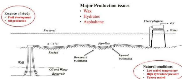
Figure 1. Schematic representation of oil-water two-phase subsea production
