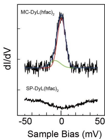
Fig. 8. STS spectra obtained for the molecules of SP-DyL(hfac) 2 (below) and the one after the electron injection, which is assumed MC-DyL(hfac) 2 . Before opening the feedback loop, the set point was V_s = -50 mV, I_t = 50 pA, and the modulation of V_{rms} = 1 mV superimposed on the sample bias. The solid lines show the fitting results.
