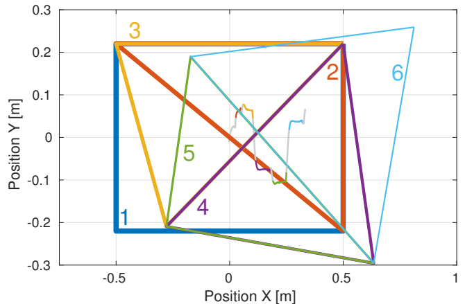
Fig. 6. Sequence of support polygons generated by the proposed algorithm. The ZMP trajectory is plotted as well, with a color that matches the corresponding polygon (grey corresponds to four-stance phases).
