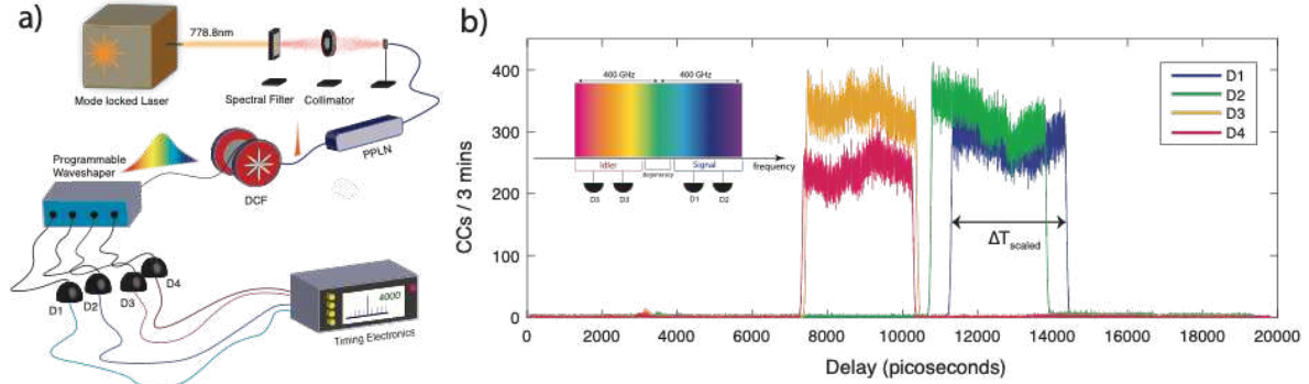
Figure 1. a) Experimental setup. b) Time-stretched replica of the signal and idler spectrum. (See text for more details)
