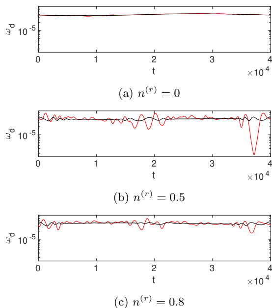
FIG. 7: The angular velocity \omega_d ( rad/\Delta t ) of the droplet front point P at the stationary regime for a quarter rotation period under the eighth-order BB virtual density method (red line) and the eighth-order improved PSM method (black line). The capillary number of the system is around 5.6 \times 10^{-3} , and the Laplace number is around 330.
