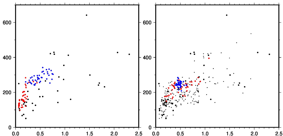
Figure 13. Scatterplot of surface chlorophyll concentration vs POC flux at 100 m depth. At 36°W, 44.25°N, on May 26, 2019. With the LETKF algorithm (left) and the MCMC sampler (right). Prior (black), augmented prior (small black dots), analysis (blue), 4-day forecast (red).
