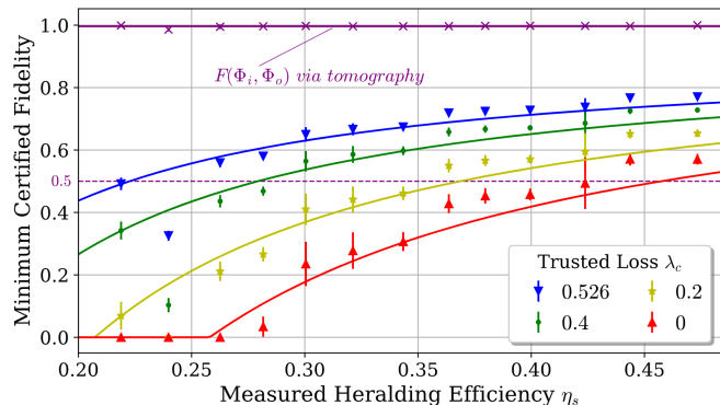
FIG. 5: Minimum fidelity F(\rho_i, \rho_o) certified via our protocol as a function of the measured heralding efficiency, tuned with a VOA, and for different trusted losses \lambda_c (colored curves). The curves are plotted by taking the average fidelity of the probe state to a Bell state \bar{F}_i , and the average of the deviation from maximum violation \epsilon , over all protocol attempts. Experimental results deviate from these curves, as F^i and \epsilon vary between experiments. Errors induced by the finite statistics are directly subtracted from the certified fidelity, as detailed in Methods (see Eqs. (28) and (29) in particular). Error bars include effects induced by the unbalance in detectors' efficiency and the propagation of errors on F^i . We also display the fidelity F(\rho_i, \rho_o) measured via quantum state tomography, for \rho_i = \Phi_i .
