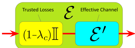
FIG. 4: Schematic decomposition of the untrusted channel \mathcal{E} , into an equivalent channel \mathcal{E}' that the protocol effectively certifies, and a trusted channel, corresponding to the characterized and homogeneous losses \lambda_c trusted by Alice.
