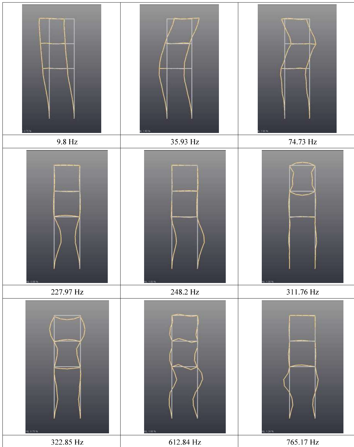
Figure 4: Identified in-plane mode shapes and eigenfrequencies
